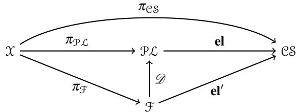
Figure 2: The co-surface graph and its friends. All rightward pointing arrows are coarsely Lipschitz, and \mathcal{D} is a quasi-isometry. Coarsely speaking, all maps are \text{Out}(\mathbb{F}) -equivariant and the diagram commutes.
