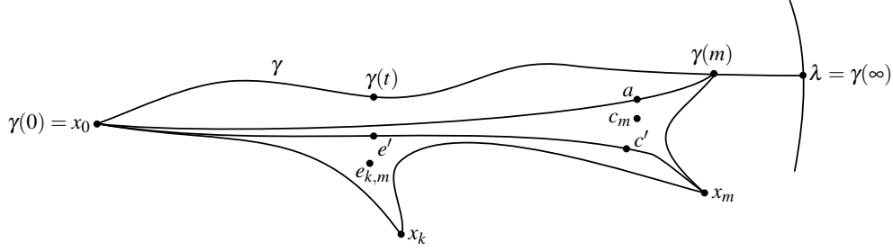
Figure 1: Proving surjectivity of \partial p .
