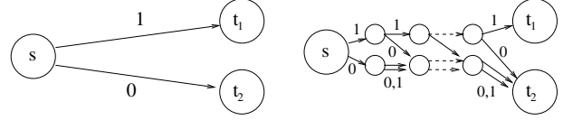
Figure 1. Replacing each (s(0), s(1)) pair with a width-2 balanced ROBP
