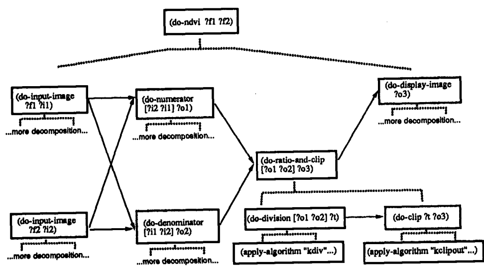
Figure 4: A simple plan fragment
