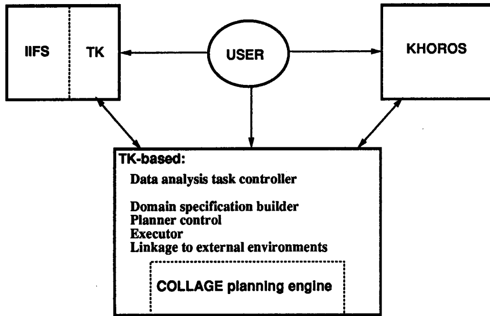
Figure 6: Creating a coherent user interaction environment
