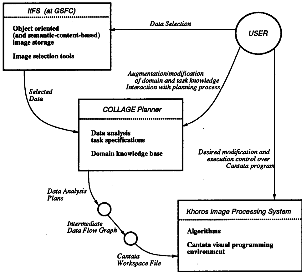
Figure 1: Integrated Planning Architecture for Data Analysis
