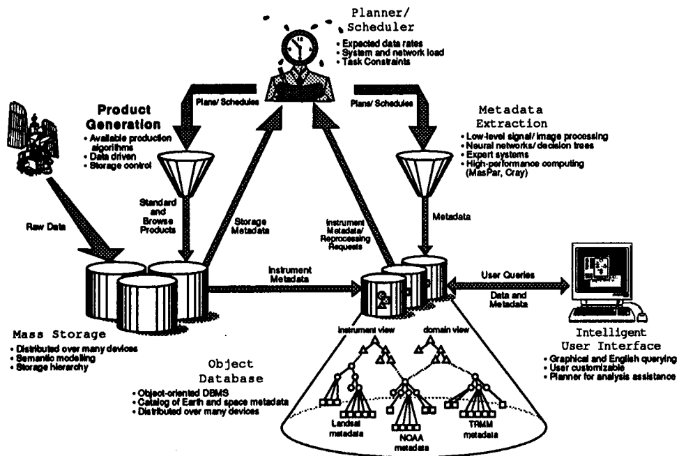
Figure 2: Intelligent Information Fusion System Architecture
