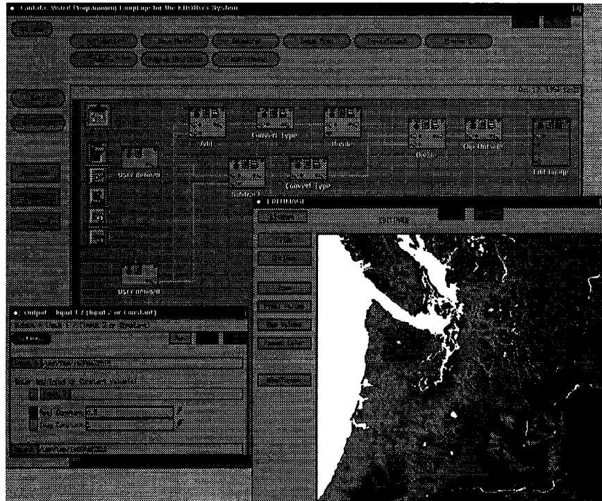
Figure 5: COLLAGE plan utilized in KHOROS/Cantata environment
