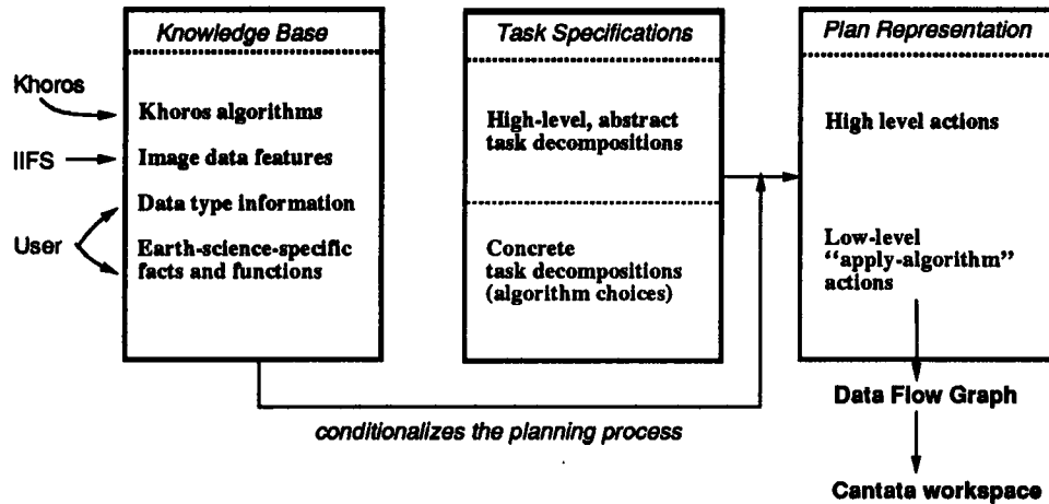
Figure 7: Structuring of information
