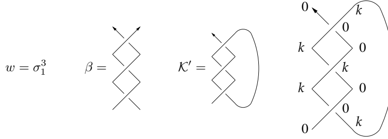
Figure 1. A word w , the corresponding braid \beta , its long closure \mathcal{K}' , and a coloring of \mathcal{K}' .
