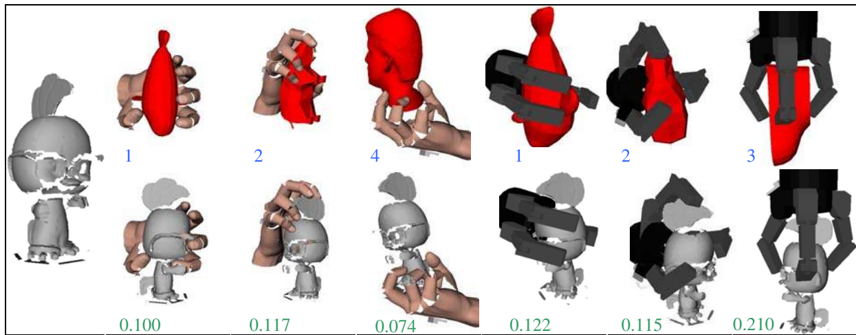
Fig. 3. Some of the grasps planned for an acquired object with holes and occlusions, using the database-backed planner with Zernike neighbors. In total 88 form closure grasps were found for the human hand and 112 for the Barrett hand.
