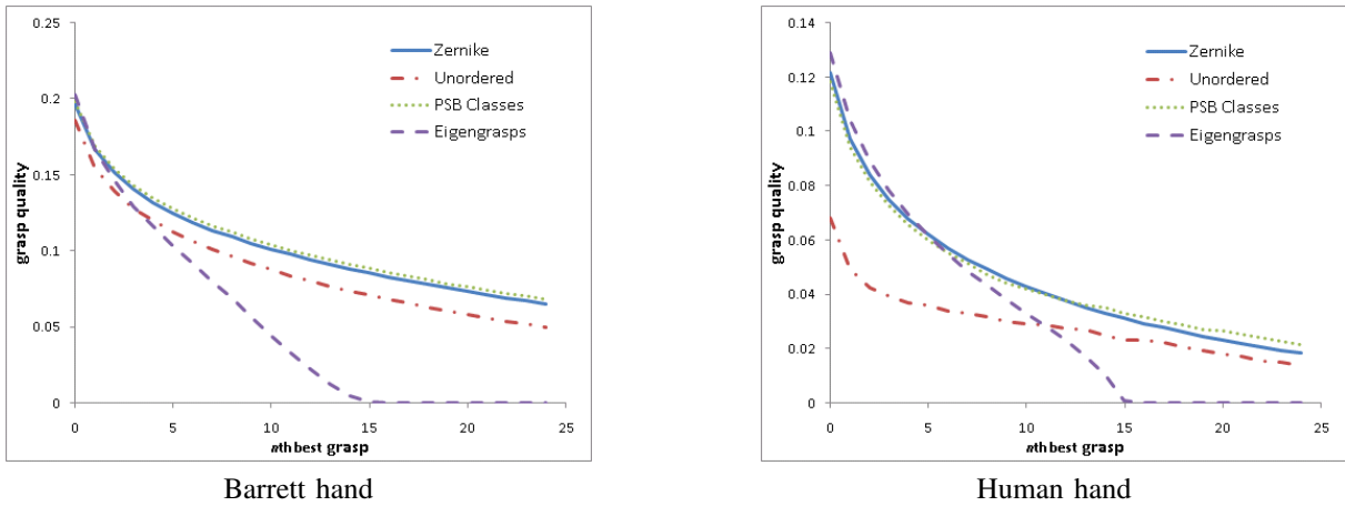
Fig. 2. The n th best grasp from database-backed grasping with 3 neighbor selection methods and from the eigengrasp planner, averaged over the 1,814 models in the database at scale 1.0. As can be seen, the information provided by shape matching is more important for the complex human hand than it is for the clawlike Barrett hand. This figure is best viewed in color.
