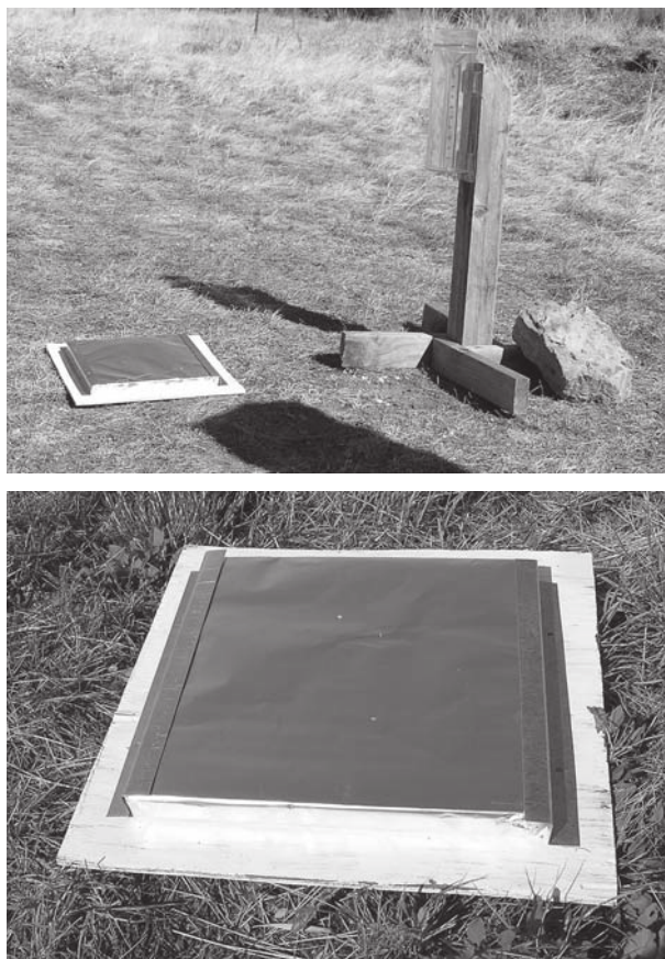
FIG. 1. (top) Instruments utilized by CoCoRaHS observers deployed for precipitation data collection: (left) 12 in. × 12 in. hail pad and (right) 4-in.-diameter rain gauge. (bottom) Close-up view of a hail pad mounted with holding brackets. The hail pad is made of styrofoam and is covered with aluminum foil.
