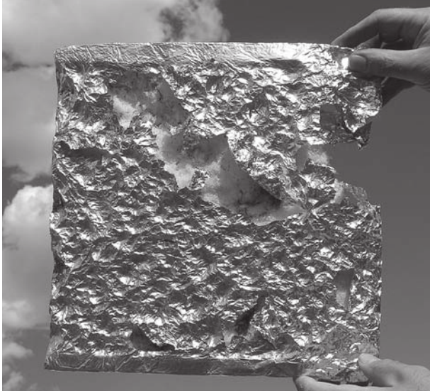
FIG. 4. CoCoRaHS hail pad after sampling 3-in. (7.6-cm)-diameter hail.
