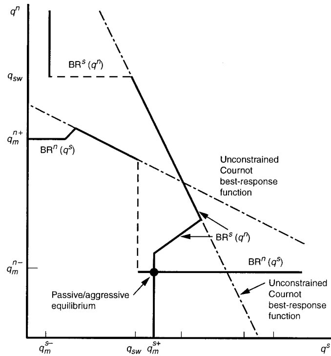
FIGURE 5 ASYMMETRIC PURE-STRATEGY EQUILIBRIUM
