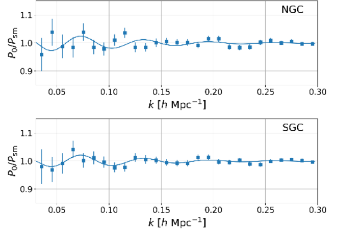
Figure 12. Isotropic BAO fit (top: NGC, bottom: SGC), in the baseline case: NGC + SGC, 0.6 < z < 1.1 , \Sigma_{\text{nl}} = 4 \text{ Mpc}/h . Both data (points with error bars from EZ mocks) and model (continuous line) are divided by the no-wiggle power spectrum.
