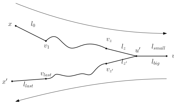
Fig. 2 A (x, x') -journey going through u
