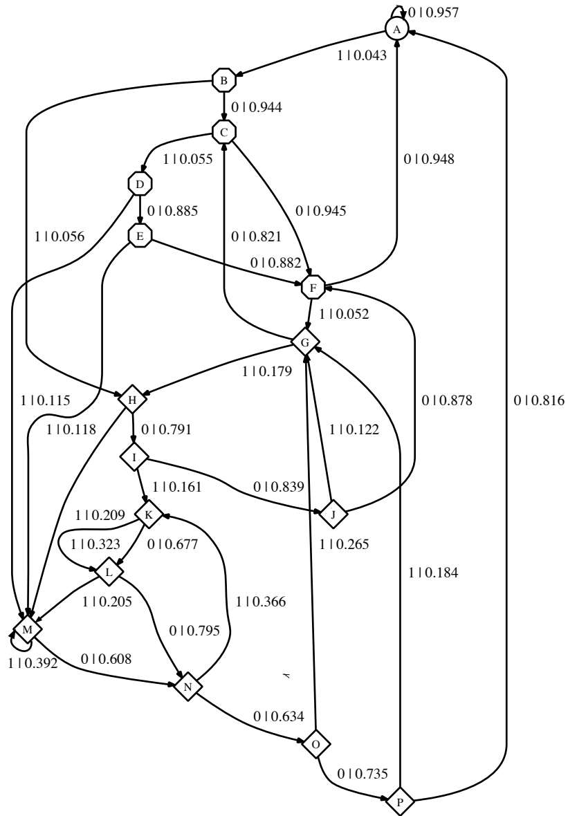
FIG. 4 16-state CSM reconstructed from 200 sec of simulation of periodically-stimulated spiking. C = 0.89 , J = 0.27 , R = 0.0007 . State A is the baseline state. States B through F (octagons) are “decision” states in which the CSM evaluates whether a spike indicates a stimulus or was spontaneous. Two spikes within 3 msec cause the CSM to transition to states G through P , which represent the structure imposed by the stimulus. If no spikes are emitted within 5 (often fewer) sequential msec, the CSM goes back to the baseline state A .
