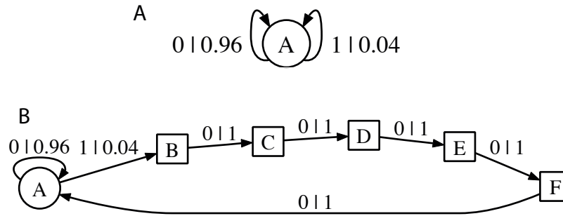
FIG. 1 Two simple CSMs reconstructed from 200 sec of simulated spikes using CSSR. States are represented as the nodes of a directed graph. The transitions between states are labeled with the symbol emitted during the transition (1 = spike, 0 = no spike) and the probability of the transition given the origin state. (A) The CSM for a 40 Hz Bernoulli spiking process consists of a single state A which always transitions back to itself, emitting a spike with probability p = 0.04 per msec. (B) CSM for 40 Hz Bernoulli spiking process with a 5 msec refractory period imposed after each spike. State A again spikes with probability p = 0.04 . Upon spiking the CSM transitions through a deterministic chain of states B–F (squares) which represent the refractory period. The increased structure of the refractory period requires a more complex representation.
