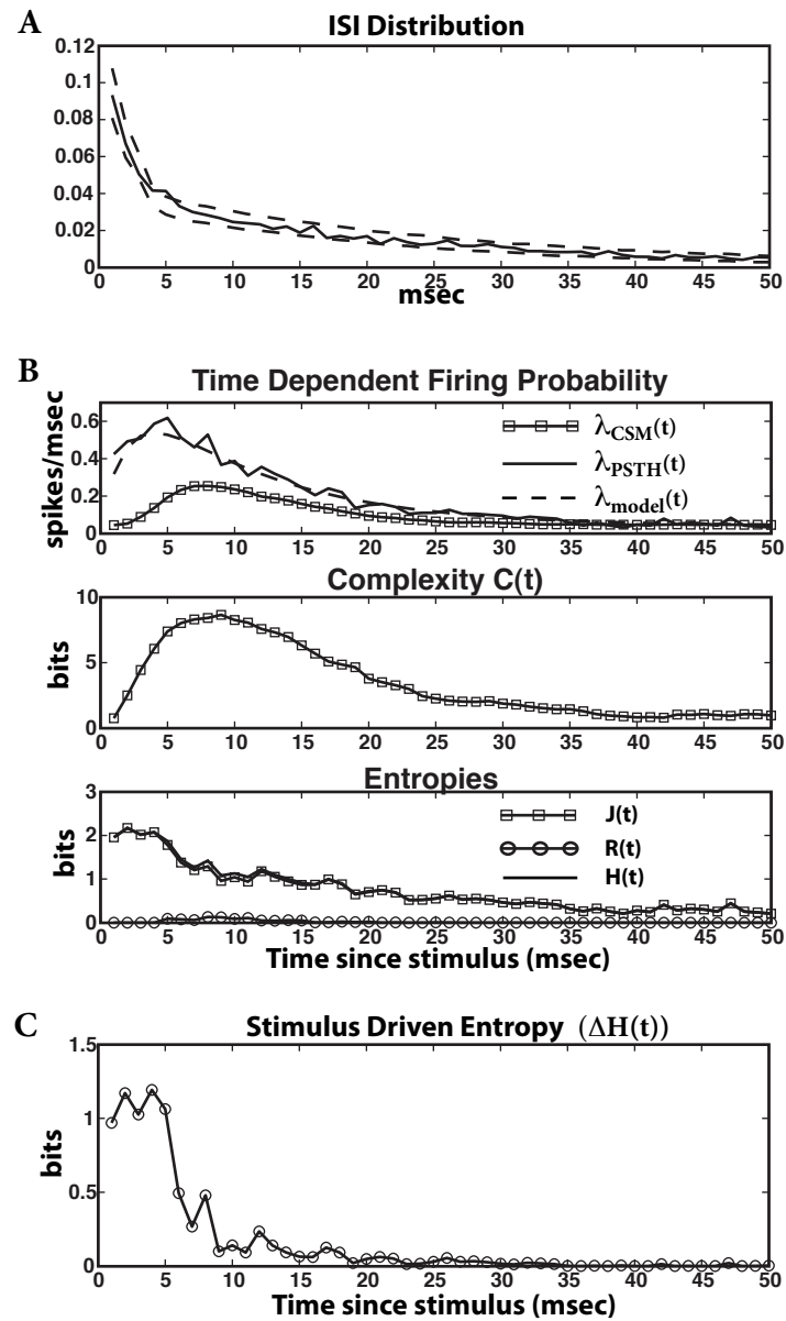
FIG. 5 Stimulus model ISI distribution and time-dependent complexity and entropies. (A) ISI distribution and 99% confidence bounds. (B) First panel: Firing probability as a function of time since stimulus presentation. Second panel: Time dependent complexity. Third panel: time-dependent entropies. (C) The stimulus-driven entropy is > 1 bit, indicating strong external drive. See text for discussion.
