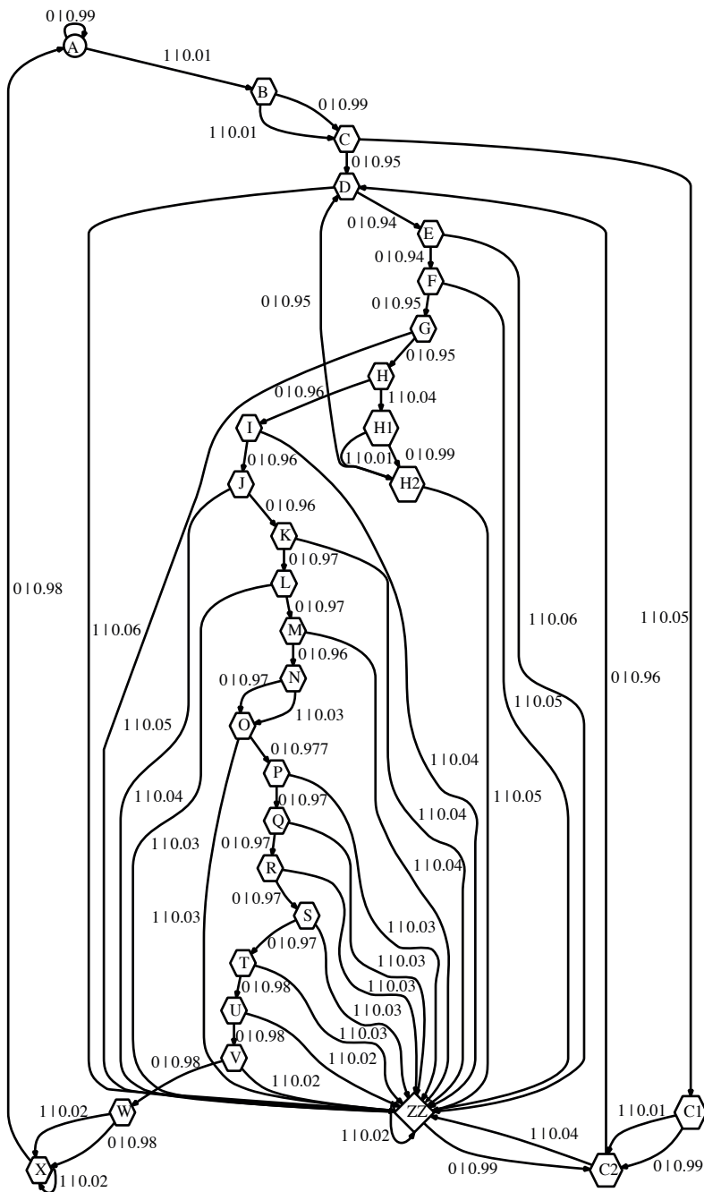
FIG. 8 29-state CSM reconstructed from 335 seconds of spikes recorded from a layer II/III barrel cortex neuron undergoing periodic (125 msec inter-stimulus interval) stimulation via vibrissa deflection. C = 1.97 , J = 0.11 , R = 0.004 . Most of the states are devoted to refractory/bursting behavior, however states “C1”, “C2” and “ZZ” represent the structure imposed by the external stimulus. See text for discussion.
