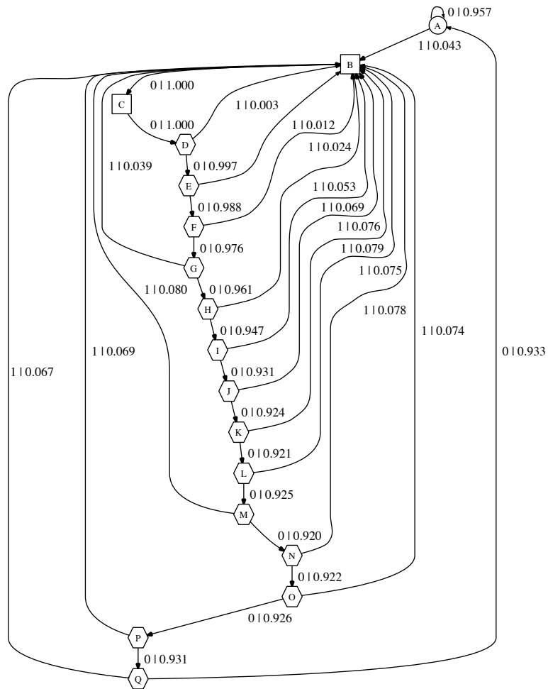
FIG. 2 CSM reconstructed from a 200 sec simulated spike train with a “soft” refractory/bursting structure. C = 3.16 , J = 0.25 , R = 0 . State A (circle) is the baseline 40 Hz spiking state. Upon emitting a spike the transition is to state B . States B and C (squares) are “hard” refractory states from which no spike may be emitted. States D through Q (hexagons) comprise a refractory/bursting chain from which if a spike is emitted the transition is back to state B . Upon exiting the chain the CSM returns to the baseline state A .
