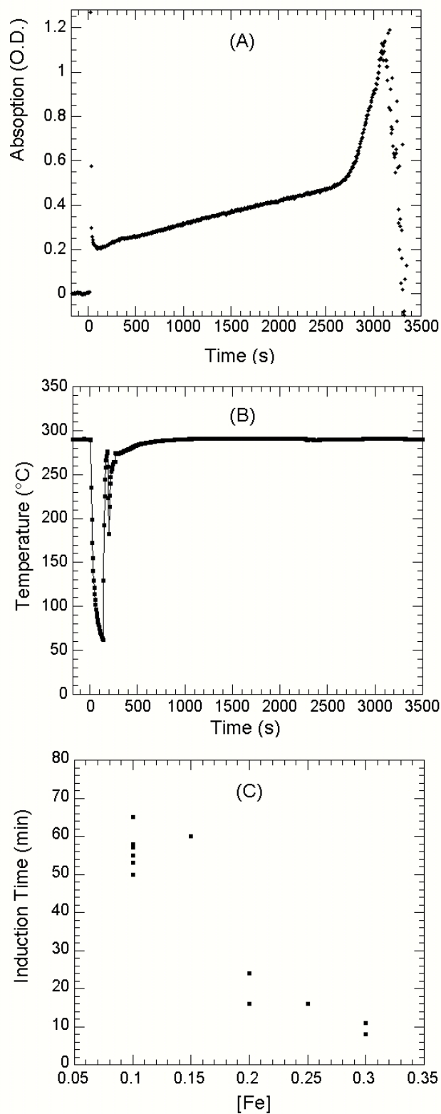
Figure 4. Optical density of the solution collected in situ at 440 nm during a typical synthesis carried out with molar ratios of \text{Fe}(\text{CO})_5 :mCPBA=1:1.5 (A) and corresponding temperature variation (B). The time=0 corresponds to the injection time; the induction time for particle formation under these conditions is about 1 hour. The dependence of the induction time on the iron precursor molar concentration is reported in (C).
