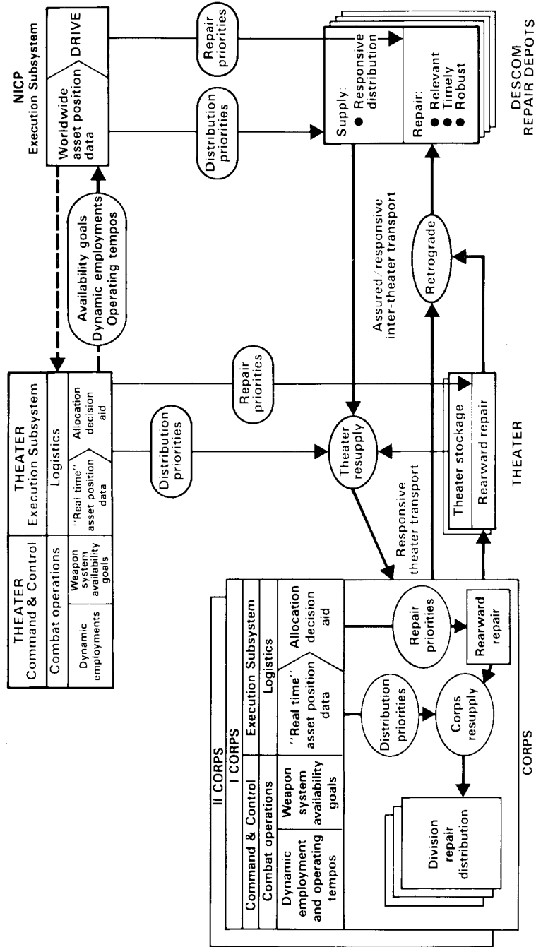
Fig. 3.1—Integrated logistics execution system
