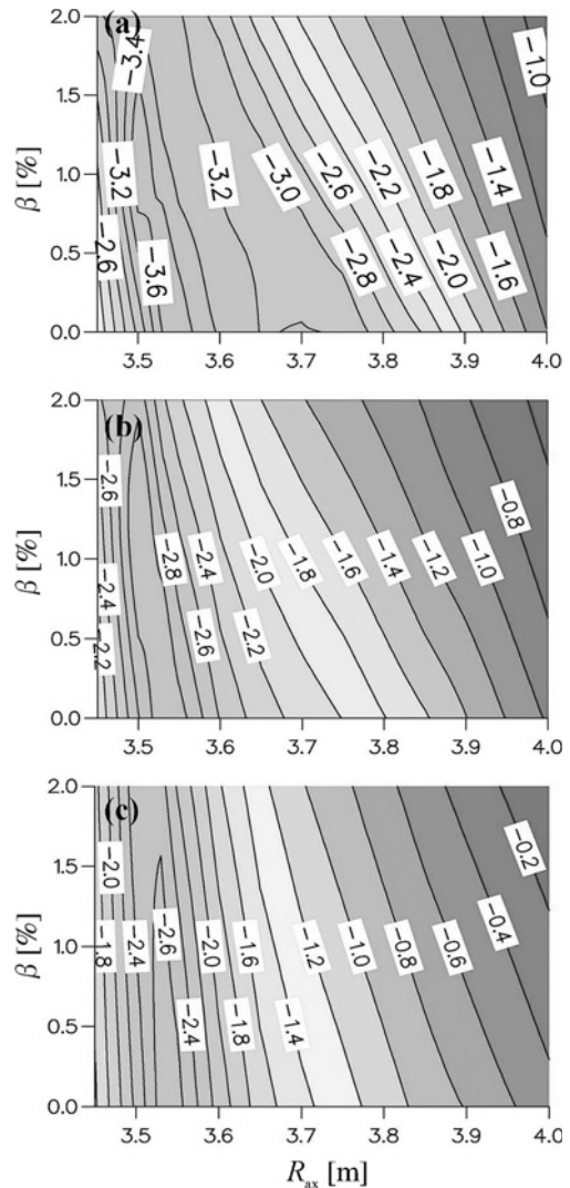
Fig. 1 Contour of \log(\epsilon_{\text{eff}}^{3/2}) on the ( R_{\text{ax}} , \beta ) plane for the radial position of (a) \rho = 0.2 , (b) \rho = 0.5 and (c) \rho = 0.8 , respectively in a wide range of LHD fixed-boundary equilibria.
