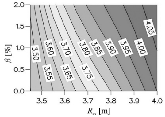
Fig. 2 Contour of the magnetic axis position on (R_{\text{ax}}, \beta) plane in a wide range of LHD fixed-boundary equilibria.
