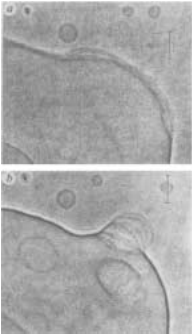
FIG. 7 Unbinding or adhesion transition as observed experimentally for a bunch of lipid bilayers in aqueous solution. a , For T \approx 22.4 °C, the membranes undulate very strongly, appearing as thick fuzzy lines. b , For T \approx 22.1 °C the membranes form a bound state, corresponding to the sharp dark line. The water between the membranes has been squeezed into the large water pocket. The bars represent 10 \mu\text{m} . (Courtesy of W. Helfrich.)
