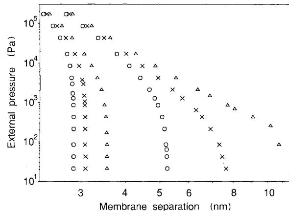
FIG. 6 Monte Carlo simulations of the separation of two interacting fluid membranes as a function of external pressure. The three curves on the right (Hamaker constants W = 5, 15 and 25 \times 10^{-21} \text{ J} ) are for room temperature; the three curves on the left represent the behaviour in the absence of shape fluctuations. The difference between these two sets of curves shows the strong renormalization of the direct interaction by shape fluctuations. \Delta , W = 5 \times 10^{-21} \text{ J} ; \times , W = 15 \times 10^{-21} \text{ J} ; \circ , W = 25 \times 10^{-21} \text{ J} .
