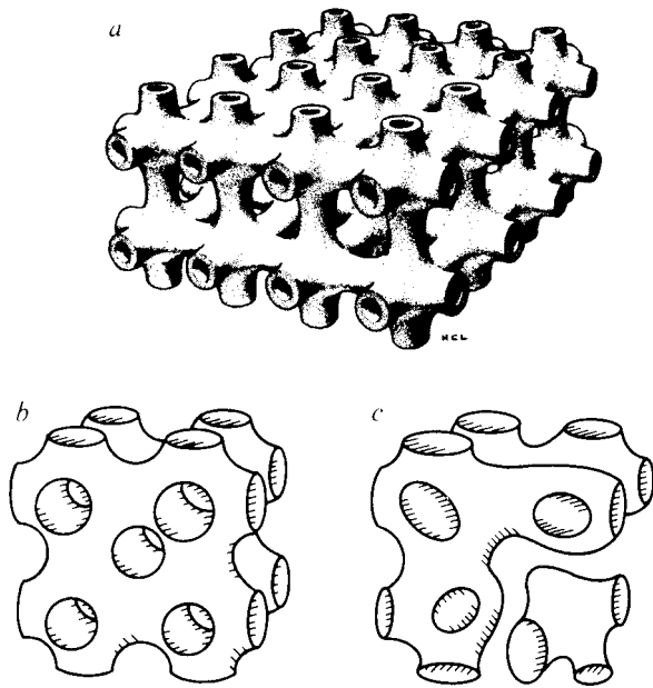
FIG. 4 Bicontinuous structures of bilayers, a, Prolamellar body as present in some organelles of plant cells 58 , b, Triply periodic minimal surface. The mean curvature vanishes for each point of this surface. c, Sponge phase, obtained by melting of the bilayer crystals shown in a and b.
