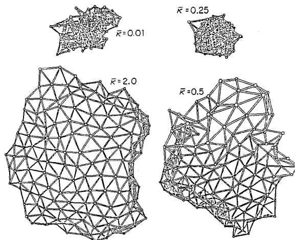
FIG. 5 Crumpling transition of a polymerized membrane with self-intersections, induced by a change in the reduced bending rigidity, \bar{\kappa} = \kappa/kT . For \kappa/kT = 0.01 and 0.25 , the membrane is crumpled; for \kappa/kT = 2.0 and 0.5 , the membrane is rough but not crumpled. The transition takes place at \kappa/kT \approx 0.33 . (Courtesy of Y. Kantor and D. R. Nelson.)
