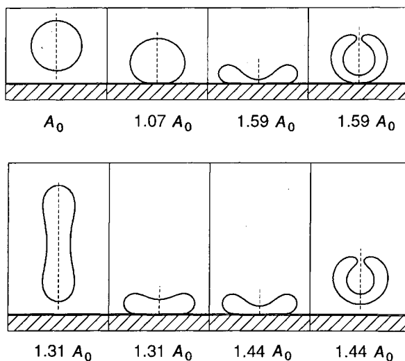
FIG. 3 Shape transformations of a vesicle interacting with a planar surface. These transformations are induced by a change in area at constant volume. The initial state is a sphere with area A_0 . The upper and the lower sequence correspond to two different contact potentials.
