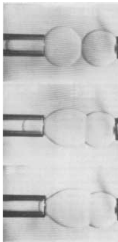
FIG. 2 Adhesion of two lipid vesicles which are brought into contact by two micropipettes. The vesicle radii are \approx 10 \mu\text{m} (courtesy of E. Evans).
