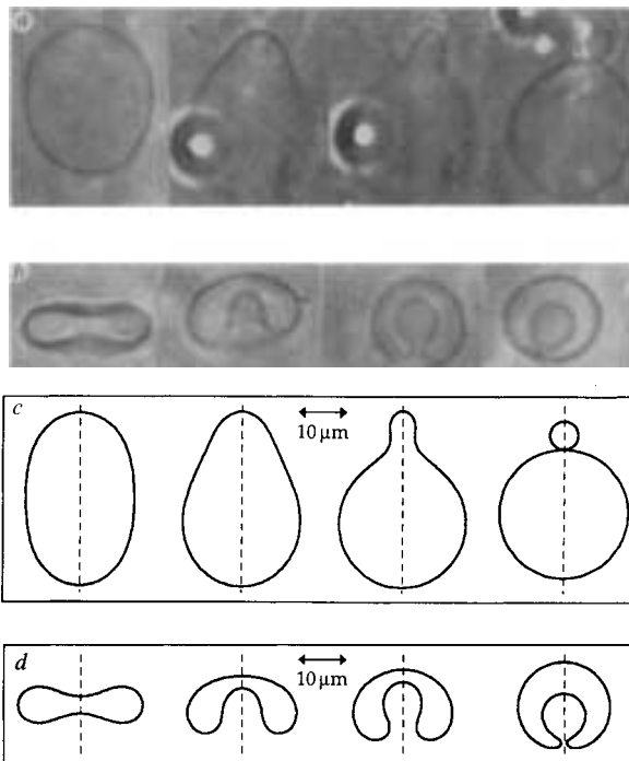
FIG. 1 Shape transformations of free vesicles induced by a change in temperature 4 . a, c , Expulsion of a small vesicle from a larger one (budding). b, d , Inverse budding ('endocytosis') via the transformation from a discocyte to a stomatocyte. The shapes are axisymmetric with respect to the broken line.
