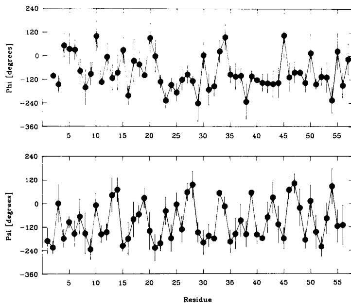
Fig. 4. Angular r.m.s. distributions of the \phi and \psi backbone torsion angles of the RDDG structures. The filled in circles ( \bullet ) are the values of the \phi and \psi angles of the mean RDDG structure and the bars represent the average angular r.m.s. deviations of the RDDG structures about the mean RDDG structure.
