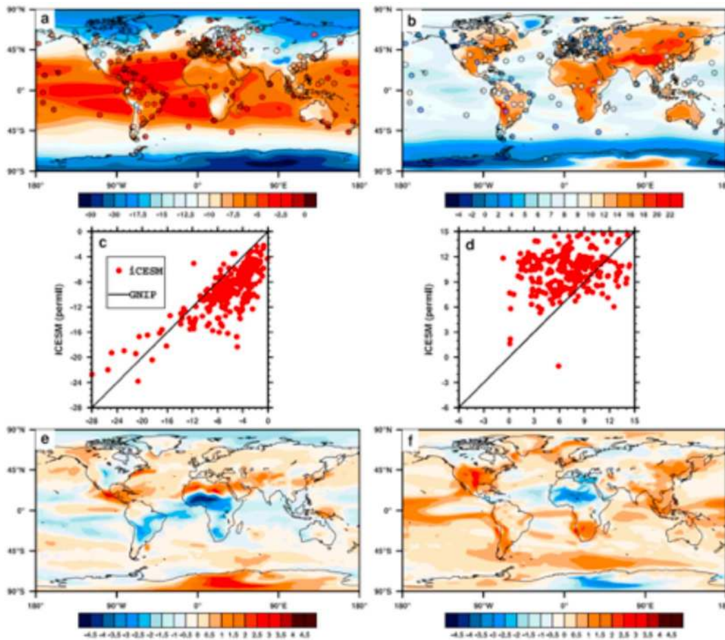
Figure 4. (a) Annual average precipitation \delta^{18}\text{O} and (b) d-excess from iCESM1.2 (contours) and GNIP (circles). Also shown are the (c) average \delta^{18}\text{O} and (d) d-excess values from the model grid cells closest to each GNIP station, compared against those GNIP values. The black line shows the values for a “perfect” match with GNIP. The differences between iCESM1.2 and iCAM5/iCLM4 with prescribed SSTs are also shown for (e) precipitation \delta^{18}\text{O} and (f) d-excess. The iCESM1.2 values were averaged over model years 1950–2005. The iCAM5 and GNIP values were the same used in Nusbaumer et al. (2017).
