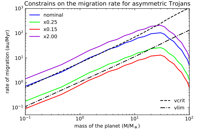
Fig. 13. Migration rates for the nominal model (blue line), the growth track 2 times faster than the nominal one (violet line) and the growth tracks 0.25 and 0.15 times the nominal one (green and red line, respectively). The black dashed line represents the critical migration rate at which L_3 and L_4 start to merge and disappear v_{\text{crit}} \approx 1.45q\Omega r (Ogilvie & Lubow 2006). The black dash-dotted line represents the lower limit for the migration rate to get an asymmetry comparable with the one observed and estimated in our simulations, that is v_{\text{lim}} \approx 0.17q\Omega r .
