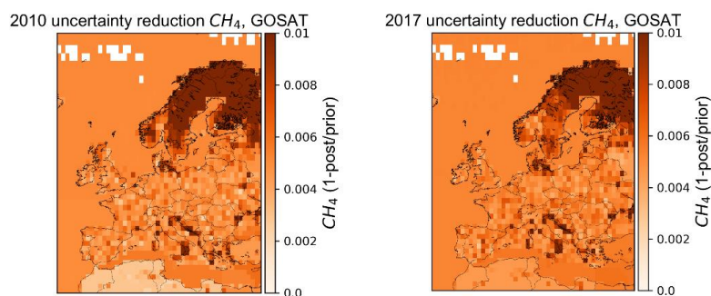
Figure 9: CTE-CH 4 GOSAT inversion run, uncertainty reduction maps computed as (1-\Delta_{\text{post}}/\Delta_{\text{prior}}) for 2010 (left) and 2017 (right).
