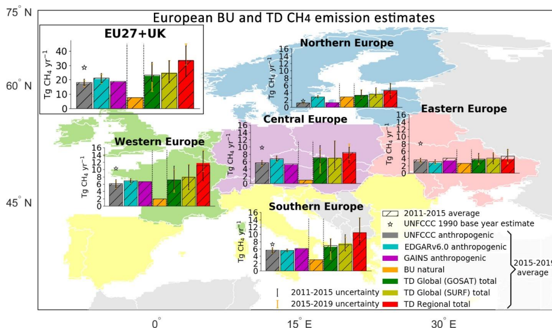
Figure 1: Five-year means (2011-2015 and 2015-2019) in total CH 4 emission estimates (excluding LULUCF) for EU27+UK and five European regions (North, West, Central, South and East non-EU). Eastern European region does not include European Russia. Northern Europe includes Norway. Central Europe includes Switzerland. The data comes from UNFCCC NGHGI (2021) submissions (grey), which are plotted with respective base year 1990 (black star) estimates, two inventories (GAINS and EDGAR v6.0), natural unmanaged emissions (sum of peatland, geological, inland waters (Reccap2) and GFEDv4.1 biomass burning emissions) and three inversion estimates: one regional European inversion (excluding InGOS unavailable for 2013-2015) and GOSAT and SURF ensemble estimates from global inverse models. The relative error on the UNFCCC value represents the NGHGI (2021) reported uncertainties computed with the error propagation method (95% confidence interval) and gap-filled to provide respective estimates for each year. Uncertainty for EDGAR v6.0 was calculated for 2015 based on the 95% confidence interval of a lognormal distribution (Solazzo et al., 2021).
