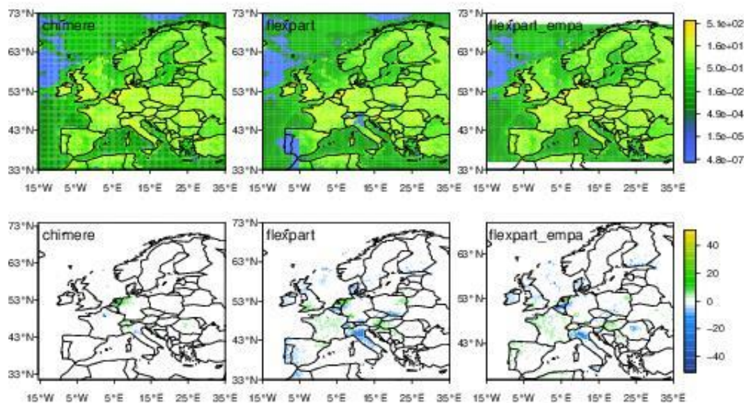
Figure 5: Posterior CH 4 fluxes averaged over 2006-2017 (g CH 4 m -2 yr -1 ) from three regional inversions, CHIMERE
