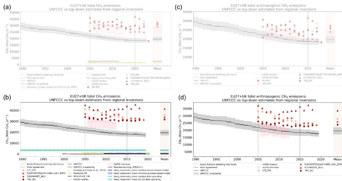
Figure 4: a) and b) Comparison of total CH 4 emissions for EU27+UK from four top-down regional inversions with UNFCCC NGHGI (grey) data and two estimates for inland waters (lakes_rivers_reservoirsprocess-based models, blue and upscaled emissions, cyan), peatlands and mineral soils(from JSBACH-HIMMELI, green), geological emissions (yellow) and biomass burning, (from GFEDv4.1, brown) as following: a) shows previous data from Petrescu et al., 2021a and b)current study; c)and d) comparison of anthropogenic CH 4 emissions from four top-down regional inversions with UNFCCC NGHGI (grey) data as following: c) previous data from Petrescu et al., 2021a and d) current study. Anthropogenic emissions from these inversions are obtained by removing natural emissions and biomass burning from total TD CH 4 emissions shown in Figure 4a,b. UNFCCC NGHGI (2021) reported uncertainties computed with the error propagation method (95% confidence interval) were calculated for each year of the time series and represents the gap-filled harmonized Member States reported uncertainty for all sectors (including LULUCF). The time series mean was computed for the common period 2005-2018 between datasets (excluding InGOS).
