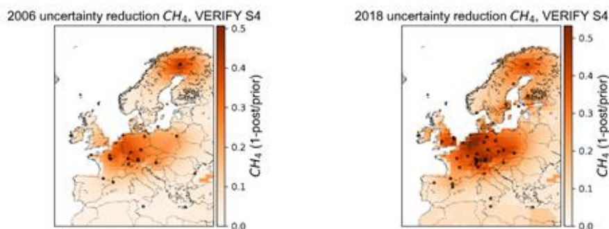
730 Figure 8: VERIFY_S4 inversion run, uncertainty reduction maps computed as (1 - \Delta_{post}/\Delta_{prior}) for 2006 (left) and 2018 (right) with different sets of observation stations.
