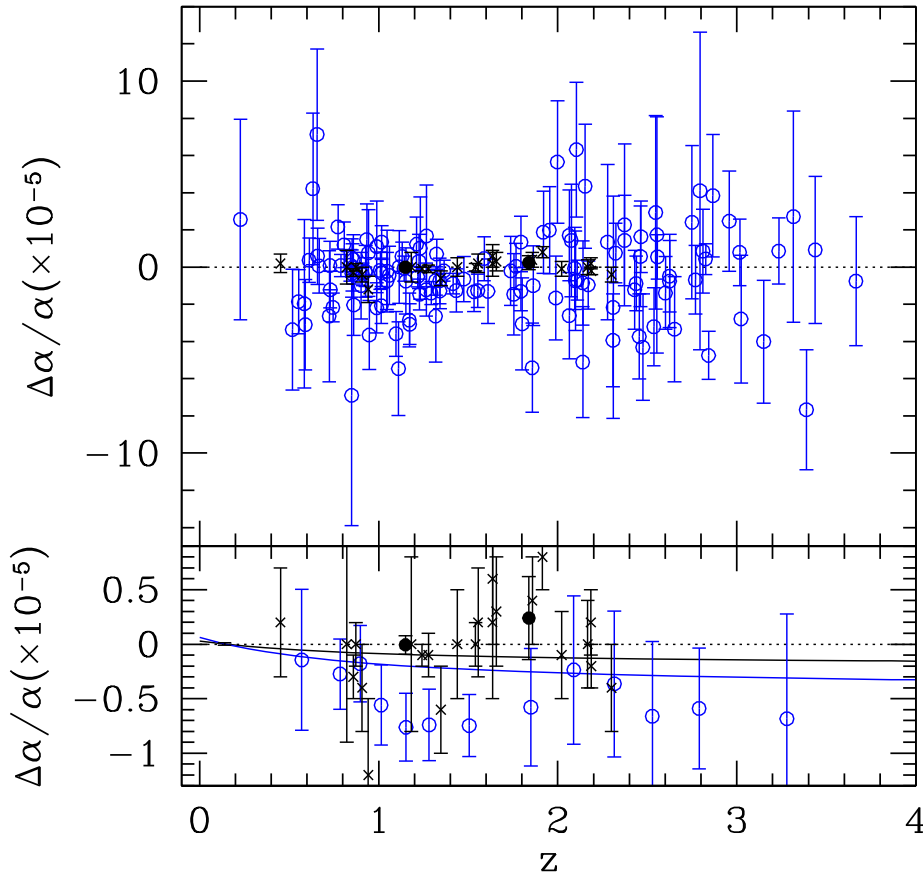
Fig. 1. (color online) The fine structure constant determined by quasar absorption lines at several redshifts. Open (blue) circles are the data from 35), 36), 38) (Keck) and crosses are from 41) (VLT) filled circles are from 44), 45) (VLT). The lower panel is the binned data of 35), 36), 38) and the value of \Delta\alpha/\alpha in each bin is the weighted mean with its associated 1\sigma error bar. The datum at z \simeq 0.14 is the Oklo bound. 18) A curve is a linear (in scale factor) fit to the data: \Delta\alpha/\alpha = 2.93 \times 10^{-7} - 2.31 \times 10^{-6}(1 - a) . A blue curve is a fit using 50) instead of 41) : \Delta\alpha/\alpha = 6.08(\pm 2.22) \times 10^{-7} - 4.85(\pm 1.46) \times 10^{-6}(1 - a) .
