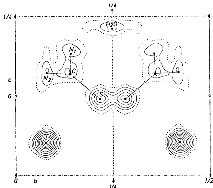
Fig. 1. Electron density projection of formamidinium disulphide diiodide monohydrate (I) along the a axis. The figure shows two asymmetric units. Contours at intervals of 10 \text{ e} \cdot \text{\AA}^{-2} for the iodide ion, 5 \text{ e} \cdot \text{\AA}^{-2} for sulphur, 4 \text{ e} \cdot \text{\AA}^{-2} for oxygen and 3 \text{ e} \cdot \text{\AA}^{-2} for the carbon and nitrogen atoms. The 3-electron line is dashed. The final atomic positions are marked with dots, and lines drawn to indicate the outline of the disulphide cation.
