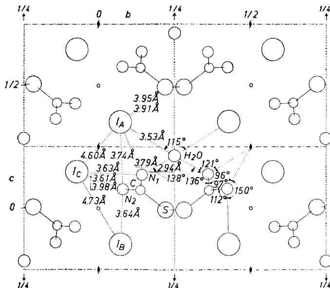
Fig. 6. The atomic arrangement in formamidinium disulphide diiodide monohydrate as seen along the a axis. Some non-bonded approaches and distances and angles relevant to the location of the hydrogen atoms are indicated.
