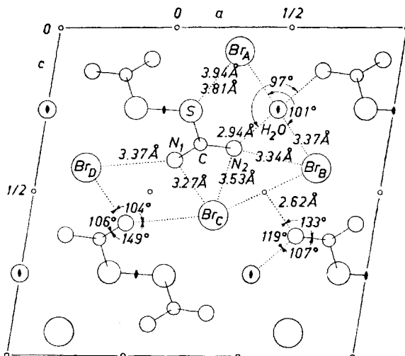
Fig. 7. A view along the b axis of the dibromide (one and a half unit cell) with interatomic approaches indicated as in Fig. 6.
