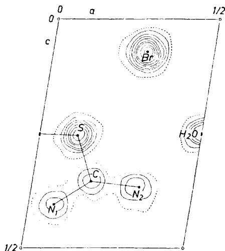
Fig. 3. Electron density projection of the asymmetric unit of formamidinium disulphide dibromide monohydrate (II) along the b axis. The 3-electron line is dashed, and contours are at intervals of 6 e \cdot \text{\AA}^{-2} for the bromide ion, 3 e \cdot \text{\AA}^{-2} for sulphur and oxygen and 2 e \cdot \text{\AA}^{-2} for carbon and nitrogen. The final atomic positions are marked with dots, and the outline of one thiourea group is drawn; the other thiourea group (not shown) of the disulphide cation lies on the other side of the twofold axis.
