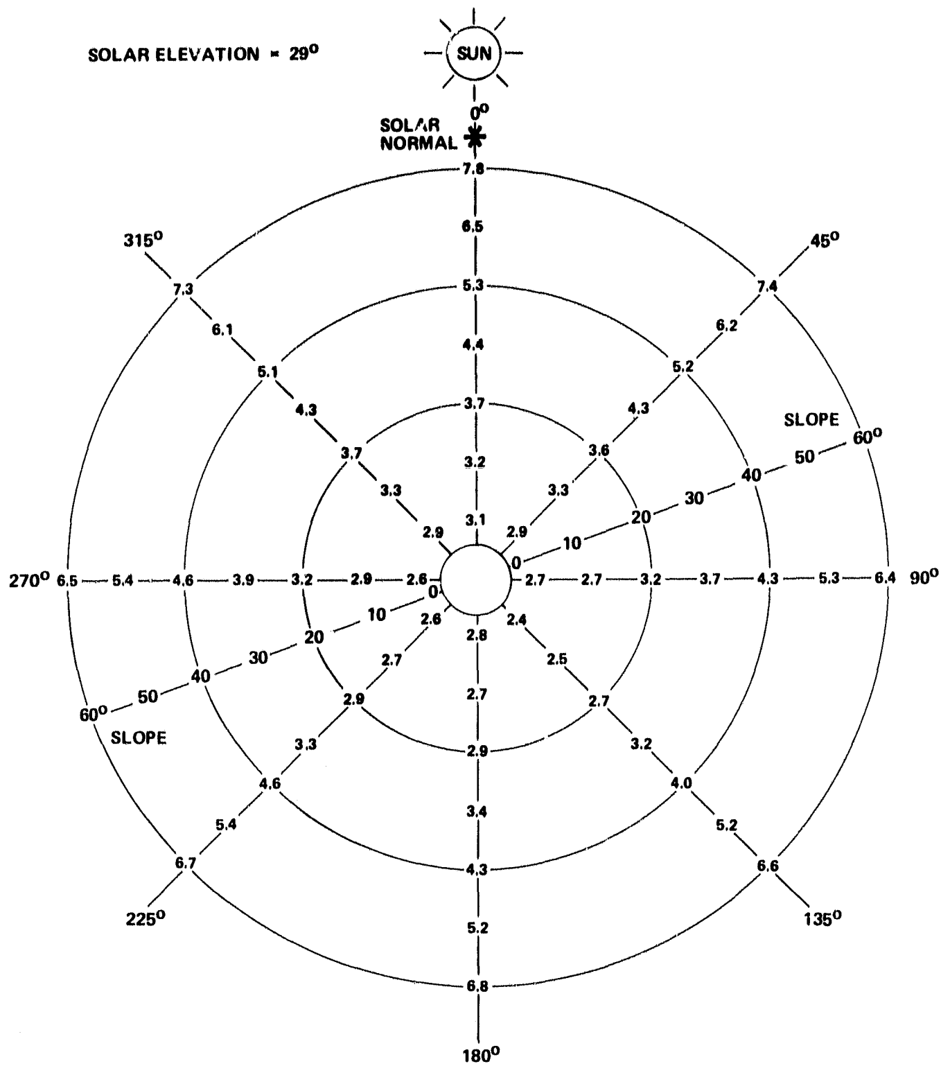
Figure 2. Diffuse Radiance ( W/m^2 - sr ) ( .76 - .90 \mu m ) Plotted By Slope and Aspect - Coarse Sand Surface
