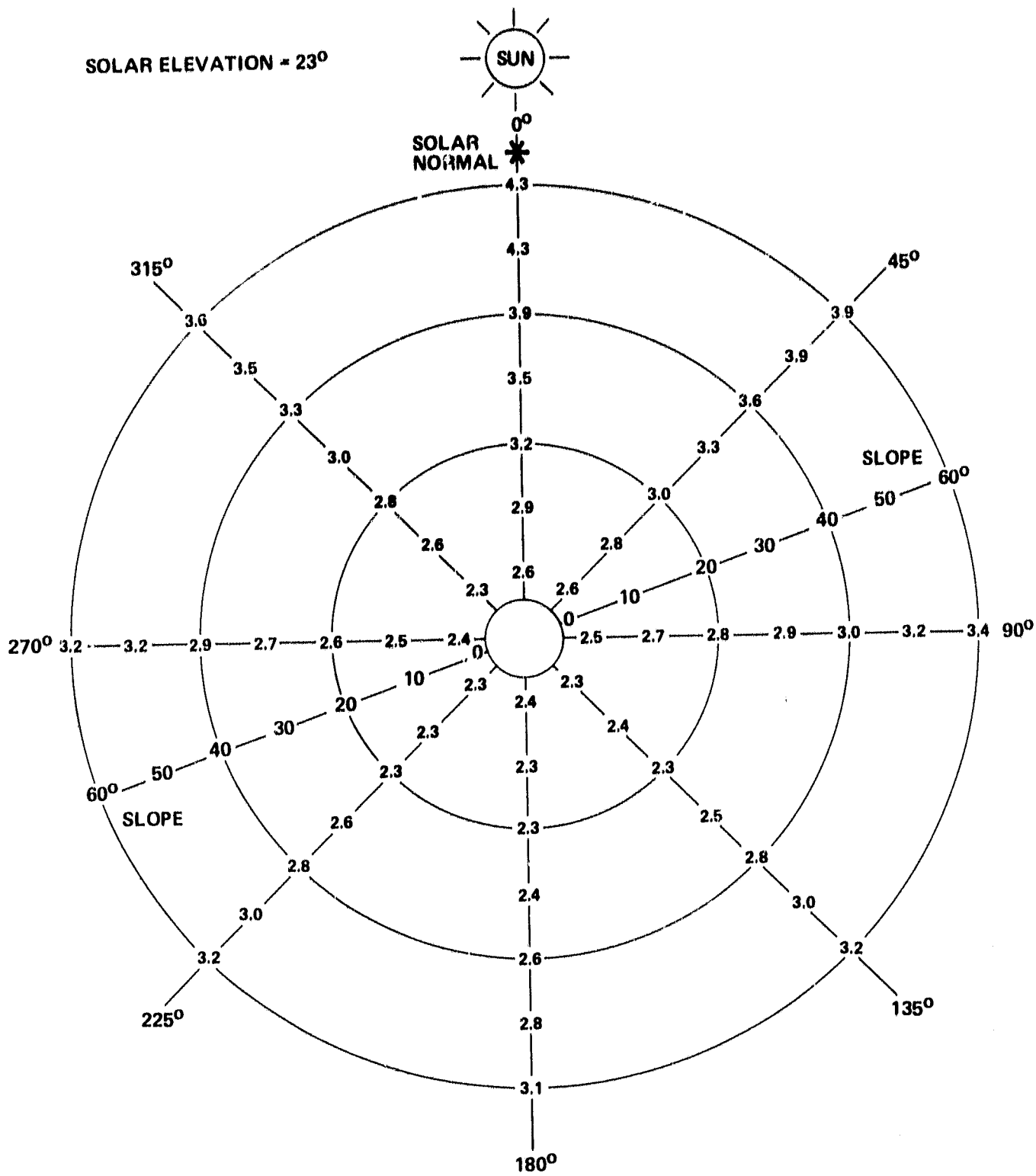
Figure 5a. Diffuse Radiance ( W/m^2 \cdot sr ) (.63 - .69 \mu m ) Plotted by Slope and Aspect - Barium Sulphate Surface
