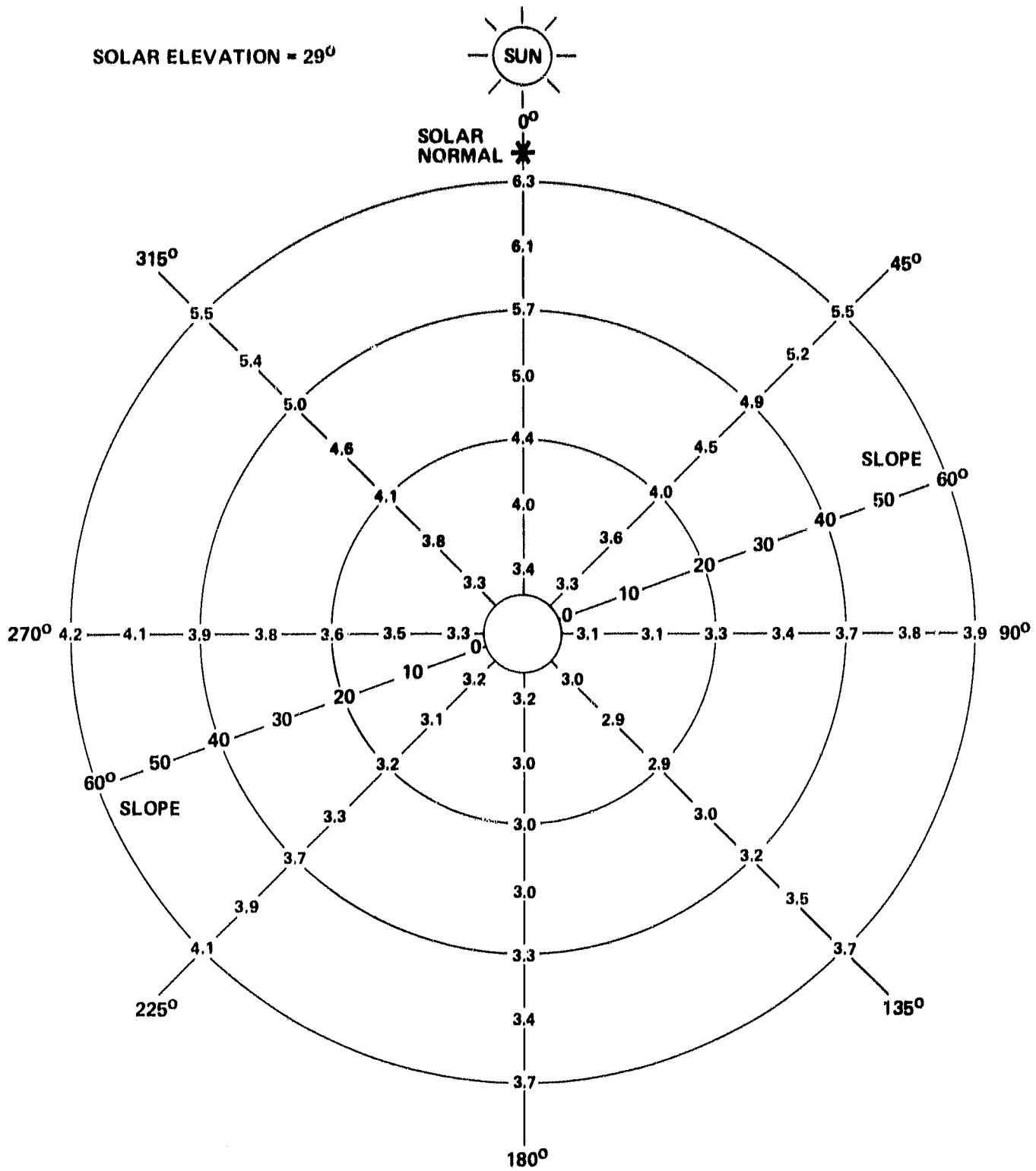
Figure 4. Diffuse Radiance ( W/m^2 \cdot sr ) ( .63 - .69 \mu m ) Plotted by Slope and Aspect - Barium Sulphate Surface
