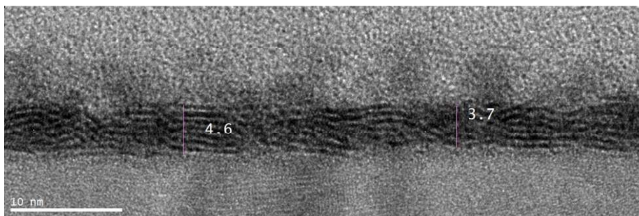
Figure 8: TEM cross-sectional image of a stoichiometric \text{WS}_2 film prepared with 14 cycles of ( \text{WF}_6/\text{N}_2/\text{H}_2\text{S}/\text{N}_2 ) of 15 s period for each pulse). The bars with the numbers indicate the thickness of the \text{WS}_2 film in nm.
