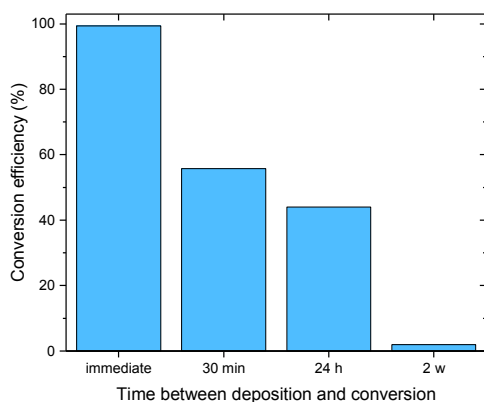
Figure 2: Conversion efficiency upon different periods between Si deposition and WF_6 conversion indicate a decreasing W amount. 100 % correspond to 2.47E15 \text{ at/cm}^2
