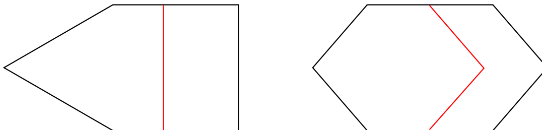
Figure 13: The red line in the convex body on the left is a minimizer. However, its image in the Steiner symmetrization of the convex body is not a minimizer. This behavior makes it difficult to relate the isoperimetric profiles of the two regions.
