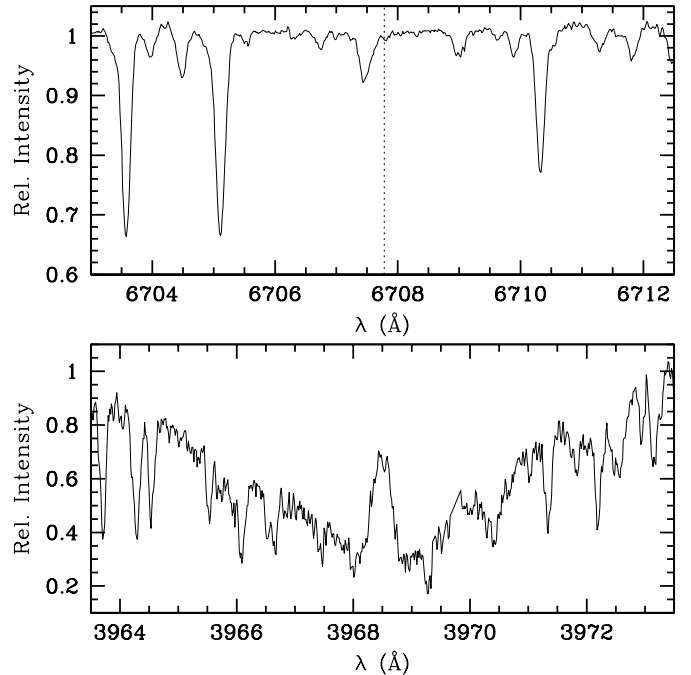
Fig. 1. Upper panel: added CORALIE spectrum in the Lithium line region for HD 41004. The plot reveals no clear Li detection for this star. Lower panel: added CORALIE spectrum in the Ca H line central region for HD 41004. The strong emission near line center suggests that the star is chromospherically active.
