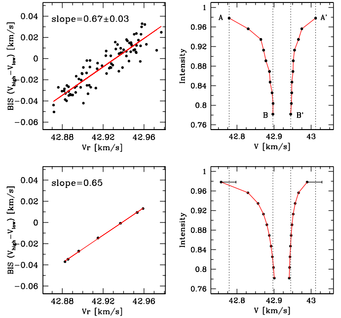
Fig. 10. Left: comparison between the observed and simulated slope of the relation between radial-velocity and BIS. Right: comparison between the shape of the bisector of the CCF for the maximum and minimum velocities. For the observed case, an average of the bisectors for the measurements corresponding to the maximum/minimum of the velocity was considered. The vertical lines are drawn just to facilitate a comparison. The error-bars drawn represent the uncertainties in the observed bisector, as well as the errors due to the fact that the real “zero” bisector is not vertical as considered in the simulations, but slightly “C” shaped (see text for more details). The parameters of the secondary CCF are the same as in Fig. 9. The velocity scale in these plots is similar to the one of Fig. 7.
