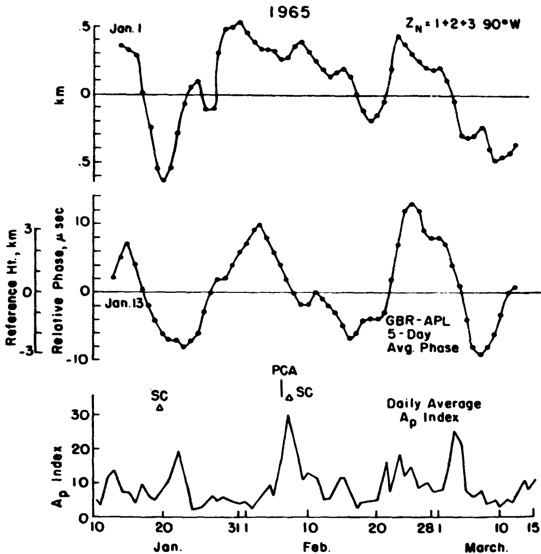
Figure 4. The 10 mb Geopotential Height Corresponding to the Sum of the First Three Fourier Harmonics at 50^{\circ}\text{N} Geographic Latitude and 90^{\circ}\text{W} Longitude, the Same GBR-APL Phase Variation from Figure 3, and the Daily Equivalent Planetary Amplitude A_p (Solar Geophysical Data, U.S. Department of Commerce).
