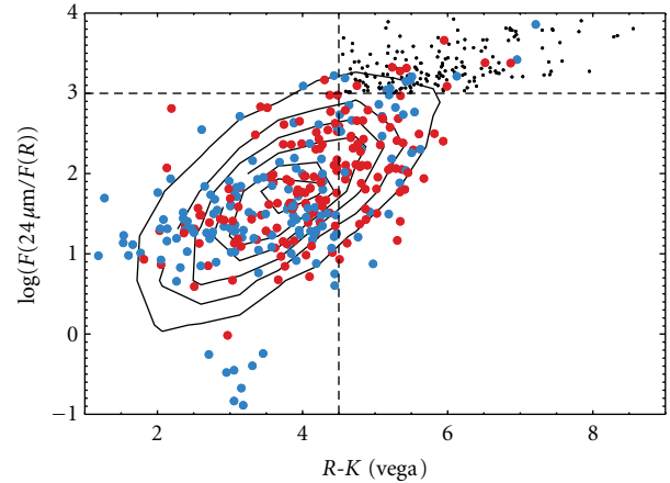
FIGURE 14: The ratio of 24-micron to R -band optical flux as a function of R - K color for the sources in the E-CDFS field [75]. Contours show the location of all the Spitzer 24 \mu m sources. Red points show the location of X-ray sources with hard X-ray spectra (hardness ratio HR > -0.3 , defined as HR = (H - S)/(H + S) where S and H are the background-subtracted counts in the soft and hard bands, resp.), while blue points have HR < -0.3 . Small black points show the 193 sources in the IR-red excess region that were not detected individually in X-rays.
