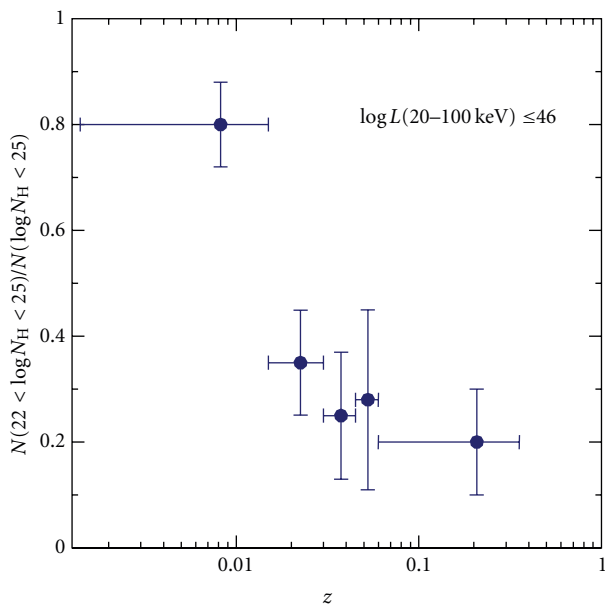
FIGURE 11: Fraction of obscured AGN ( N_H > 10^{22} cm ^{-2} ) as a function of redshift for a sample of AGN selected at high energies from INTEGRAL observations, as shown by Malizia et al. [68]. All of these sources have X-ray luminosities lower than 10^{46} erg s ^{-1} . The remarkably strong decline in this fraction at z \sim 0.015 is likely due to selection effects and not intrinsic to the AGN population. That the fraction of CT AGN in the first bin is \sim 20\% , in contrast to the \sim 5\% found overall suggests that current hard X-ray surveys are not sensitive enough to observe CT AGN beyond z \sim 0.01 . This will improve dramatically with NuSTAR [69].
