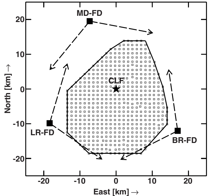
Figure 1. Layout of the Telescope Array experiment. This figure shows the 507 surface detector counters deployed on a 1.2 km grid. Fluorescence telescopes overlook the surface detector at three sites called Middle Drum (MD) on the north, Long Ridge (LR) on the southwest, and Black Rock (BR) on the southeast. The Central Laser Facility (CLF) is situated in the center of array, equidistant from all three fluorescence detectors.
