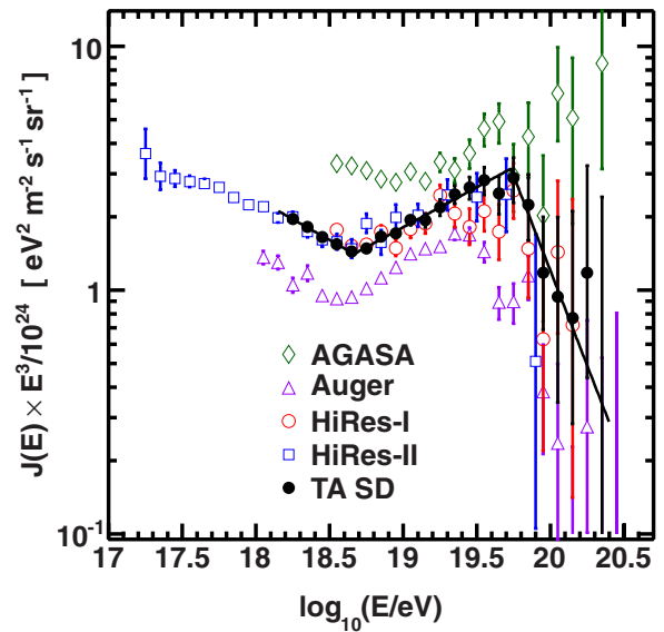
Figure 5. Cosmic-ray flux multiplied by E^3 . The solid line shows the fit of the TA SD data to a broken power law.
