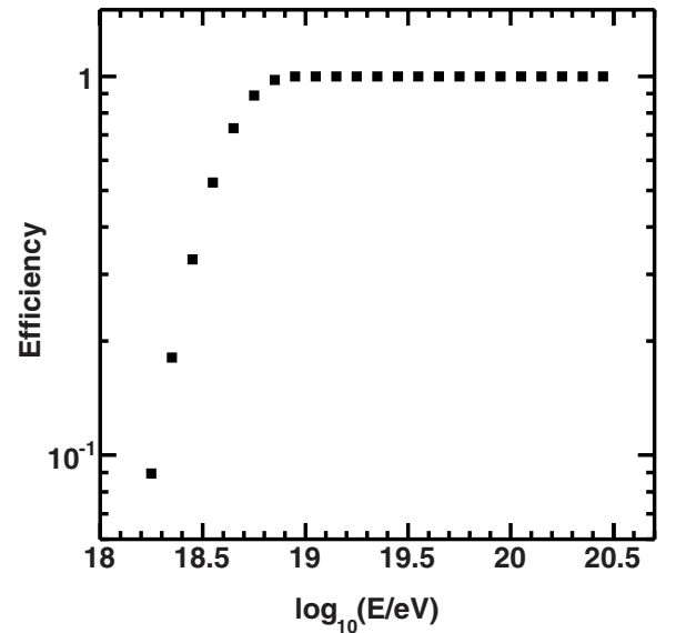
Figure 3. Efficiency as a function of energy. Both trigger and reconstruction effects are included.
