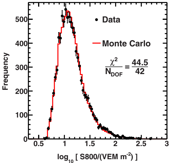
Figure 2. Data and MC comparison of the event S(800) distributions. The reduced \chi^2 is 1.06, indicating a good agreement.
