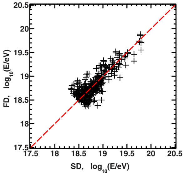
Figure 4. Energy comparison between the TA SD and FD after the 27% normalization has been applied to the SD.
