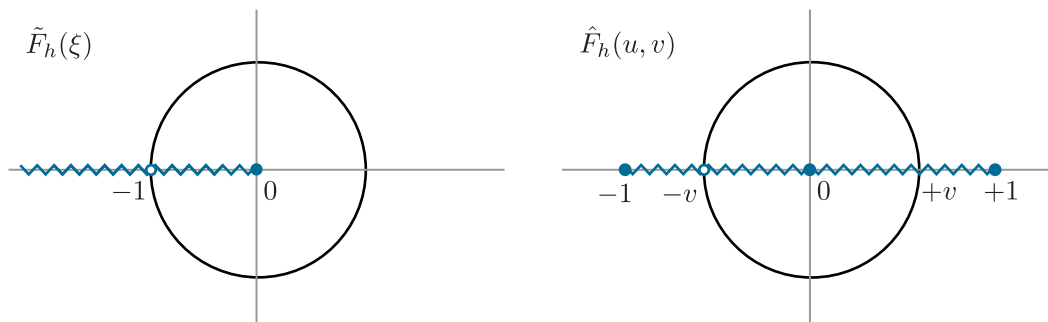
Figure 7. Illustration of the analytic structures of the functions \tilde{F}_h(\xi) (left) and \hat{F}_h(u, v) (right).
