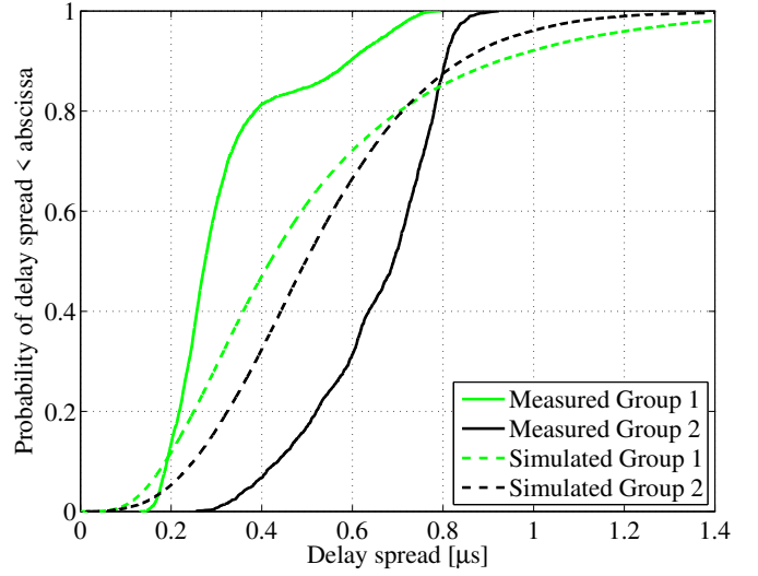
Fig. 4. Delay spreads of the measured and simulated omnidirectional antenna responses for groups 1 and 2.
