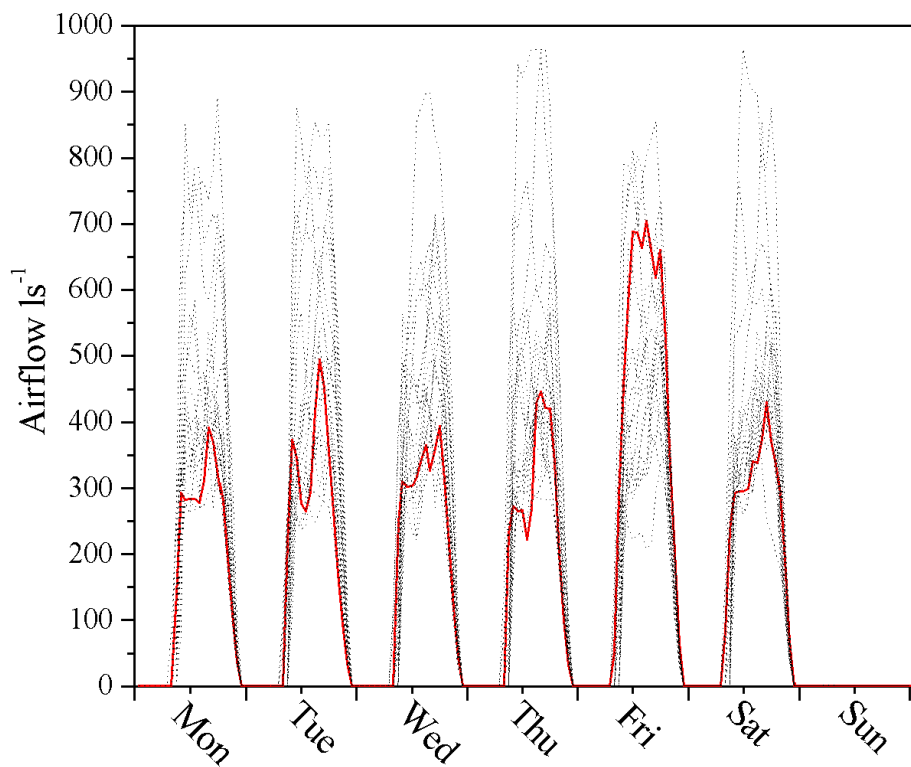
Figure 9 Plot of airflow magnitude for a typical week in summer for the TRY (red) and the 19 other observed weather years used to compile the TRY (black dash). The construction details and week considered are the same as displayed in figure 7, a list of the years used can be found in table 4.
