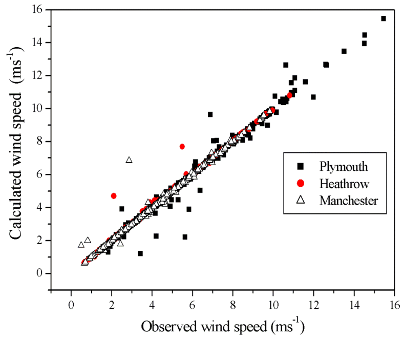
Figure 1 Observed mean daily wind speed for three locations against calculated mean daily wind speed reconstructed from PET. The correlation of the data is high with R^2 > 0.99 for all three data sets.
