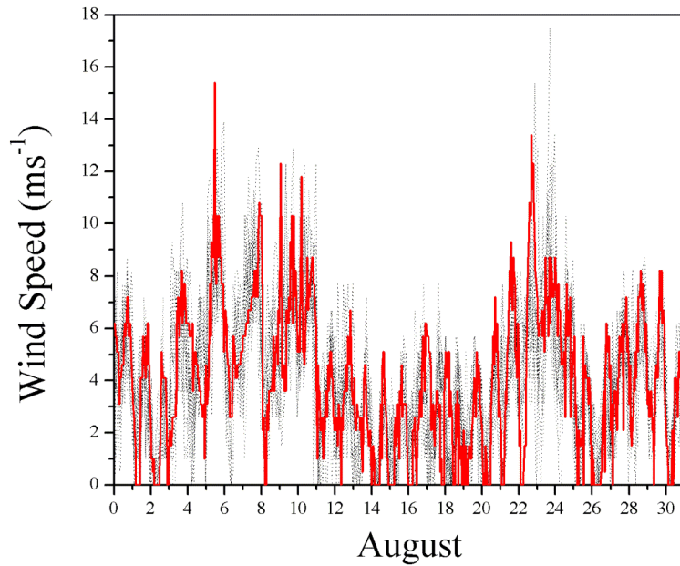
Figure 4 Plot of 15 possible wind time series (black dash) and the observed wind time series from the TRY (solid red line) for the month of August.
