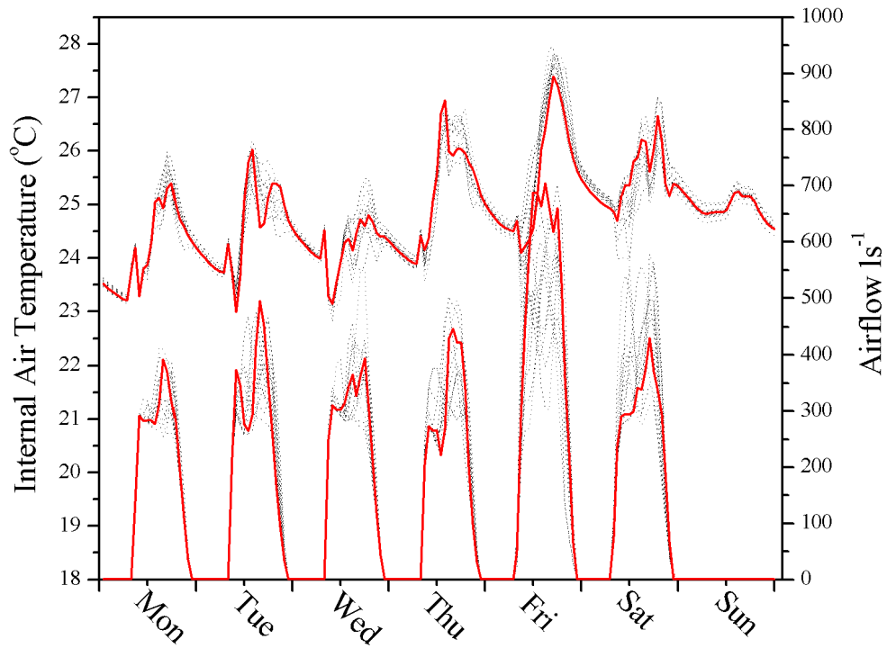
Figure 7 Plot of air temperatures (top) and airflow magnitude (bottom) for a typical week in summer for the TRY (red) and the 15 calculated wind fields (black dash) for a large open plan office. Note the windows are only open during occupied hours when the internal air temperature is > 24^{\circ}\text{C} .
