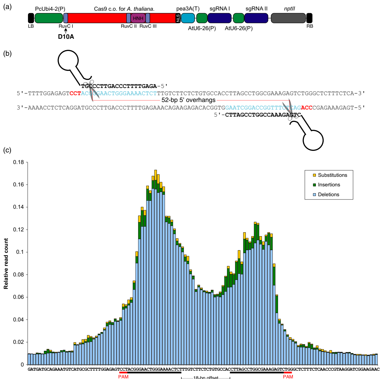
Figure 3. Targeted mutagenesis by Cas9 paired nickases.
