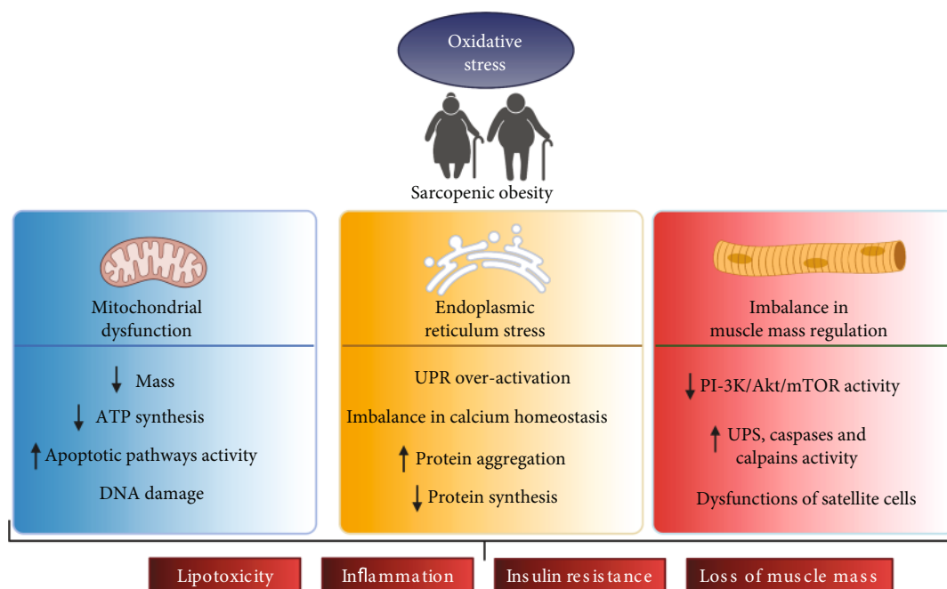
FIGURE 2: Oxidative stress in sarcopenic obesity. In older people, oxidative stress (Os) favors sarcopenia and obesity through mitochondrial dysfunction, endoplasmic reticulum (ER) stress, and imbalance in muscle mass control. Mitochondrial dysfunction in sarcopenia is induced by Os due to mitochondrial DNA damage and impaired mechanisms for repairing DNA ability, impaired capacity to remove dysfunctional mitochondria, decreased mitochondrial quantity and quality, and impaired capacity to generate ATP to activate the apoptotic pathways. ER stress and Os are caused by an increase in adipose tissue, chronic inflammation, and insulin resistance, all of which are characteristics of obesity and aging. ER stress induces Os, favoring unfolded protein response (UPR) overactivation, imbalance in calcium homeostasis, increased protein aggregation, and decreased protein synthesis. Imbalance in muscle mass control occurs because Os increases the catabolic activity and decreases the anabolic pathway in muscle mass control. Os reduces protein synthesis due to the reduced activity in phosphatidylinositol 3-kinase (PI3K)/serine-threonine kinase (Akt)/mammalian target of rapamycin (mTOR). Os increases the activity of the ubiquitin-proteasome system (UPS) and activates muscle proteases such as caspases and calpains. Finally, due to Os, satellite cells' quantity and regenerative function decline with age and obesity. Mitochondrial dysfunction, ER stress, and imbalance in the muscle mass control pathways induce lipotoxicity (Lptx), chronic inflammation, IR, and loss of muscle mass, affecting physical function and independence in sarcopenic obesity. Abbreviations: Os: oxidative stress; ER: endoplasmic reticulum; UPR: unfolded protein response; PI3K: phosphatidylinositol 3-kinase; Akt: serine-threonine kinase; mTOR: mammalian target of rapamycin; UPS: ubiquitin-proteasome system (UPS); Lptx: lipotoxicity.
