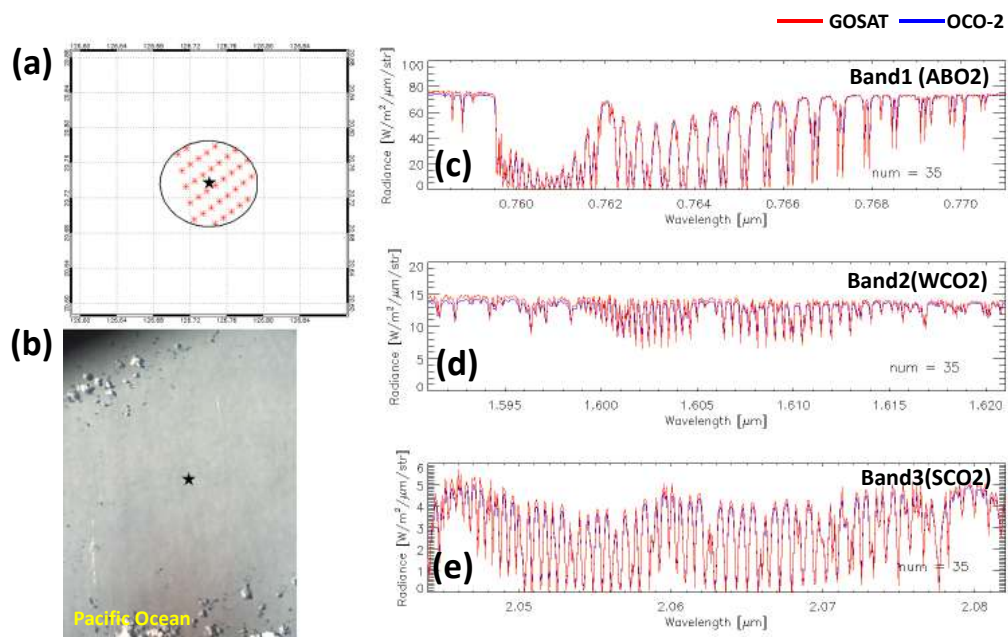
Figure A1. The spectral comparison between glint GOSAT and glint OCO-2 over the Pacific Ocean at 20.74^{\circ}N , 126.74^{\circ}E on 25 June 2015 with the GOSAT high gain. (a) The GOSAT footprint and OCO-2 matched-up pixels; the black line, the black star and the red dots represent the GOSAT IFOV, the center of the GOSAT IFOV and the OCO-2 observation points within GOSAT IFOV, respectively; (b) The GOSAT camera image from CAM bore sighted with TANSO-FTS. The spectral comparison of (c) ABO2; (d) WCO2 and (e) SCO2 bands. Red and blue lines represent the GOSAT and OCO-2 spectral radiances, respectively.
