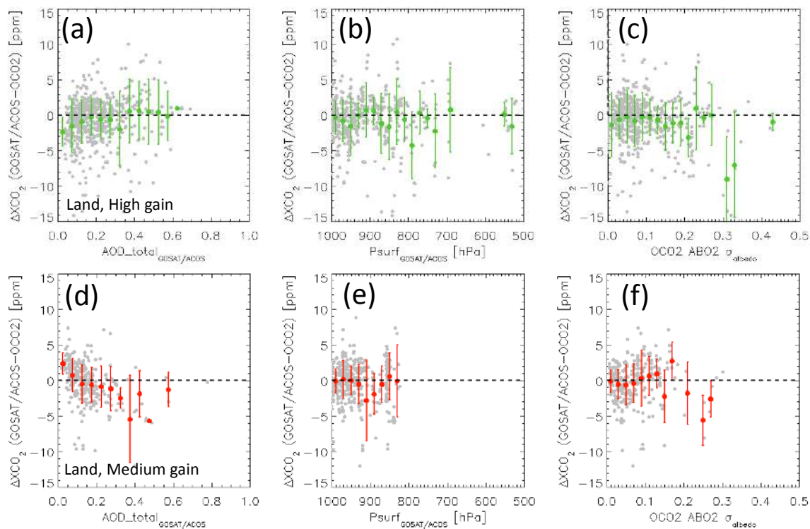
Figure 9. \Delta XCO_2 as a function of (a) GOSAT/ACOS retrieved AOD at 0.755 \mu\text{m} ; (b) GOSAT/ACOS retrieved surface pressure and (c) OCO-2 ABO2 \sigma_{albedo} over land with high gain. The lower panels (d–f) show same parameters as the above panels over land with medium gain. All match-up data were plotted with gray marks. The green and red plots and bars are the average value and standard deviation within each bin. The bin sizes are (a) 0.05; (b) 20 hPa and (c) 0.02. The upper panel shows over land with high gain and the lower panel shows medium gain.
