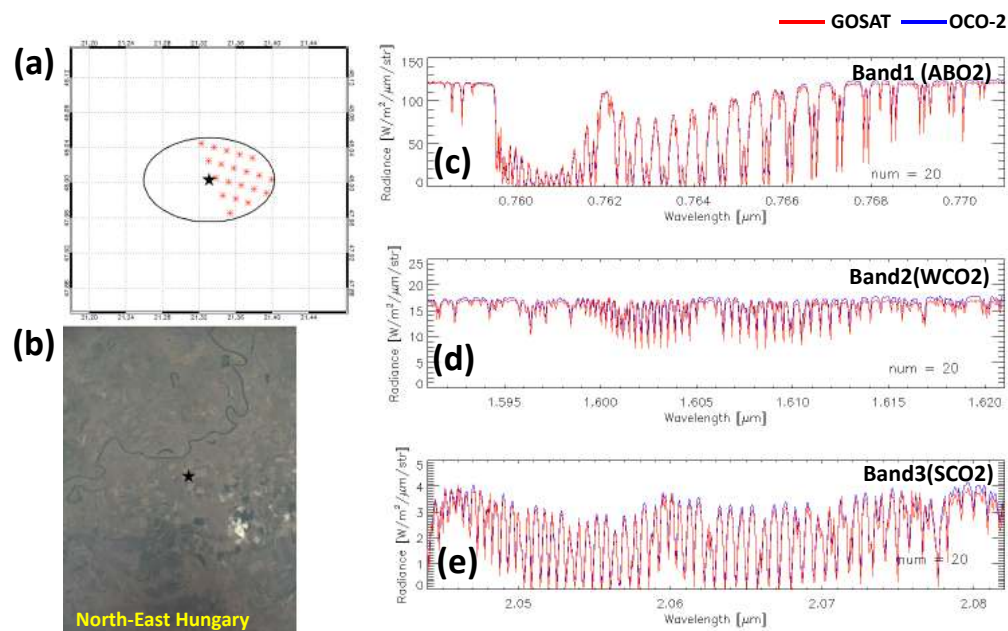
Figure A2. The spectral comparison between glint GOSAT and glint OCO-2 over a farm area in North-East Hungary at 48.0^{\circ}N , 21.33^{\circ}E on 9 June 2015 with GOSAT high gain. The plots are same as Figure A1.
