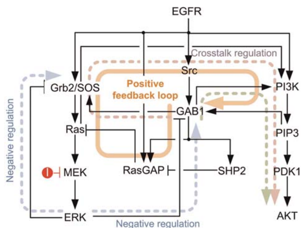
Figure 5 The reorganization of signal flux evoked by the MEK inhibitor treatment. Sandy brown-colored line indicates the newly activated route of EGF signal in response to MEK inhibition, which leads to the sustained activation of Akt. Light blue-colored line denotes the negative feedback loops which are disrupted by MEK inhibitor and light green-colored line shows the nominal route of Akt activation.
