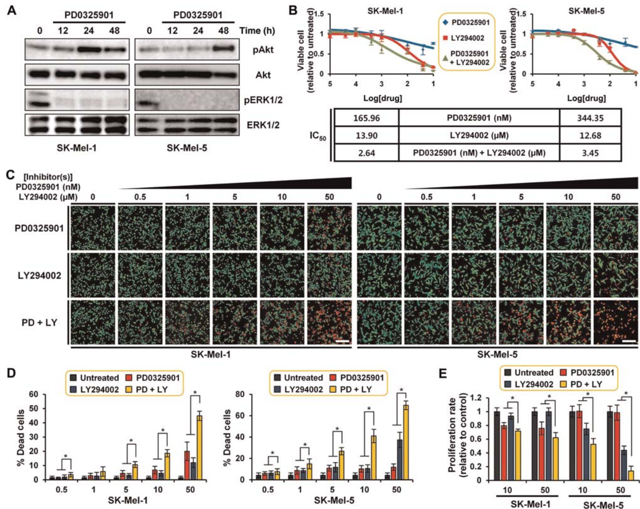
Figure 3 Combined blockage of PI3K-Akt activation shows the synergistic effects suggesting the role of PI3K pathway for the resistance to MEK inhibitor in BRAF-mutant melanoma cells. (A) Western blotting analysis of SK-Mel-1 and SK-Mel-5 following the treatment with PD0325901 (50 nM). Time point is indicated above the phospho-Akt. (B) SK-Mel-1 and SK-Mel-5 cells were treated with the indicated concentrations for 48 h and cell viability was determined. Cell viability is shown relative to the untreated control. The IC_{50} for PD0325901 or LY294002 alone and in combination are shown in a tabular form. (C) Live/dead assays of SK-Mel-1 or SK-Mel-5 cells treated with the indicated concentrations of PD0325901 or LY294002 alone or in combination for 48 h. The cells were double stained with Calcein AM and ethidium homodimer-1 (EthD-1). The Calcein AM and EthD-1 mixture show live cells in green and dead cells in red, respectively. Scale bar represents 20 \mu m. (D) Quantitative measurements of dead cell percentage. Data represent the mean \pm SD ( n > 10 , at least >2000 cells were counted). *P < 0.001 . (E) Cell number was counted after 48 h from the treatment of each inhibitor alone and in combination. The proliferation rate is shown relative to the untreated control. Data represent the mean \pm SD ( n > 10 ). *P < 0.001 .
