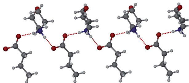
Fig. 5 The X-ray structure of BuA· 6 showing two different hydrogen bonding interactions.
