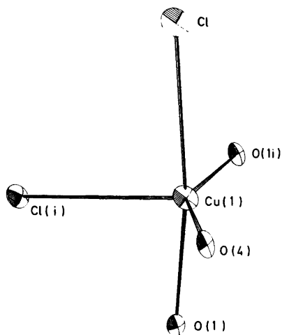
Fig. 3. Fivefold coordination of Cu(1) in form of a trigonal bipyramid: \text{Cu}(1)\text{O}_3\text{Cl}_2 .
