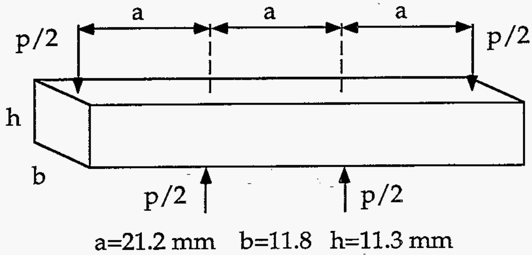
Figure 2: Loading configuration of four-point bending specimens.
