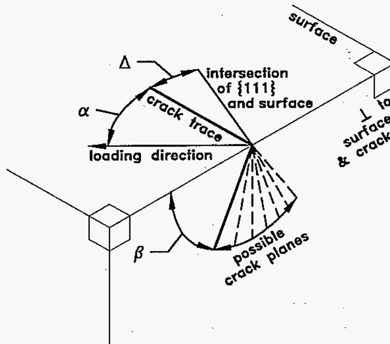
Figure 3: Diagram of the angle \alpha between the crack trace and the tensile direction, the angle \beta between a given plane and the plane of the surface, and an angular deviation \Delta between observed crack lines and one intersection of a \{111\} plane with the surface.
