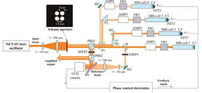
Fig. 15. (Color online) The experimental setup of the wavefront dividing four-beam combined laser. PB1 and PBS2 = polarizing beam splitters; HWP1 and HWP2 = half wave plate; P1, P2, and P3 = 45° prisms; BS = beam splitter; W = wedged window; FR1, FR2, FR3, and FR4 = Faraday rotators; C1, C2, C3, and C4 = concave mirrors; PZT1, PZT2, and PZT3 = piezoelectric transducers.
