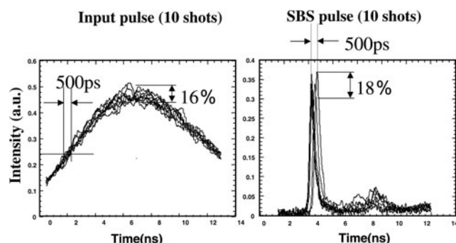
Fig. 28. The time fluctuation of input pulses and SBS compression pulses.
