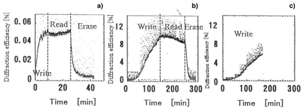
Fig. 51. Temporal evolution of volume holographic gratings in a scheme of two-step writing with 1.06- \mu\text{m} recording pulse and 532-nm gating pulse at incident energy of (a) 7 mJ, (b) 1 mJ, and (c) 0.3 mJ.
