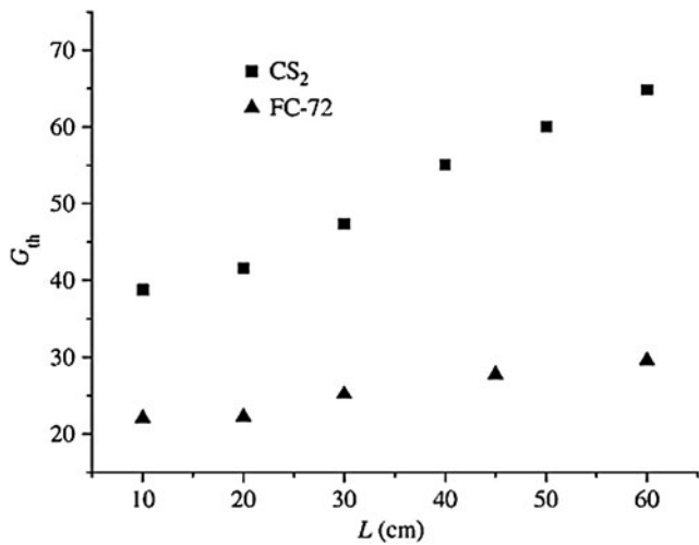
Fig. 59. G_{\text{th}} versus L .
