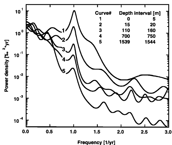
Figure 3. MEM power spectra for detailed \delta^{18}\text{O} profiles demonstrating, for five different levels in the GRIP deep core; the presence of the weak annual \delta^{18}\text{O} cycle by the spectral peaks is observed at 1 cycle/yr. The effect of smoothing by diffusion is manifested in the drastic lowering of the power densities at higher frequencies.
