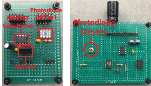
(a) Transmitter
