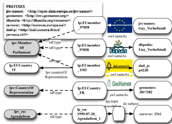
Figure 5. Examples of links to and from LinkedEP : inlinks from JRC-Names to LinkedEP MEPs, outlinks from LinkedEP MEPs to DBpedia and the Italian parliament, from LinkedEP countries to GeoNames, and from agenda items to the Eurovoc thesaurus.
