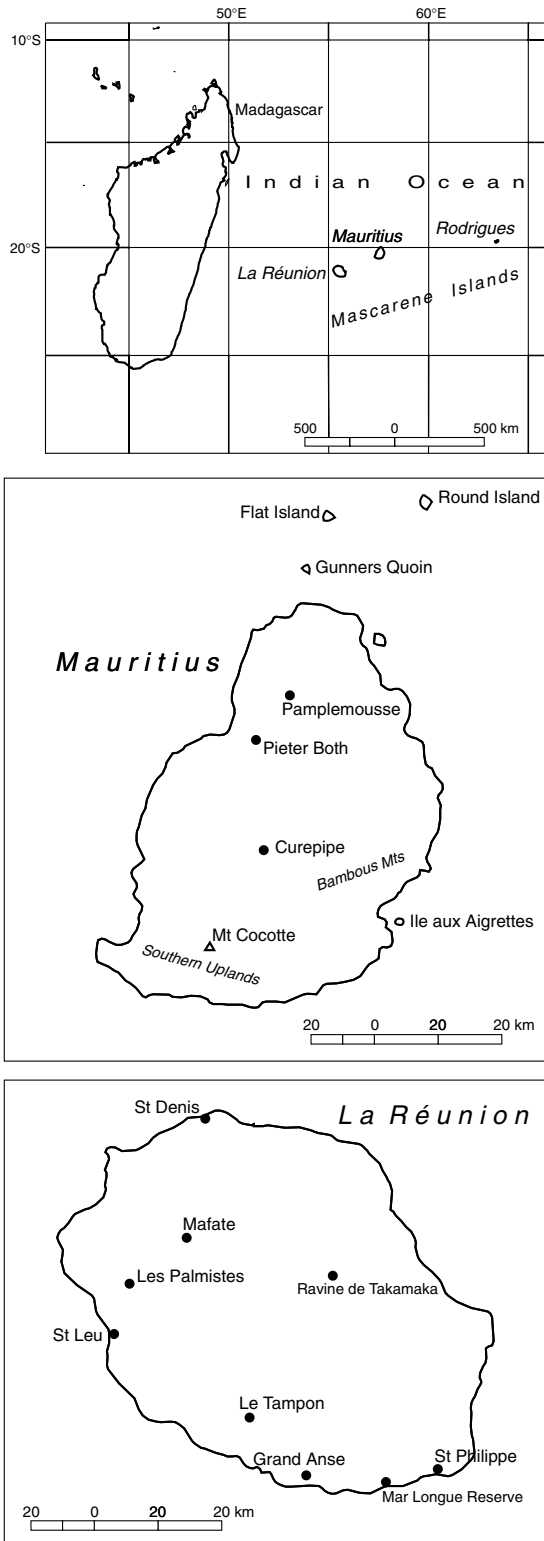
Fig. 1 The location of the Mascarene Islands of La Réunion (a French Overseas Department), and Mauritius and Rodrigues (together the Republic of Mauritius) to the east of Madagascar in the south-east Indian Ocean, and Mauritius and La Réunion with locations and islands mentioned in the text.
