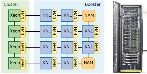
(a) Sketch of the Cluster-Booster architecture as implemented in the DEEP-ER project (KNL: Knights Landing; NVM: non-volatile memory; NAM: network attached memory). (b) Picture of the DEEP-ER prototype, at JSC.
