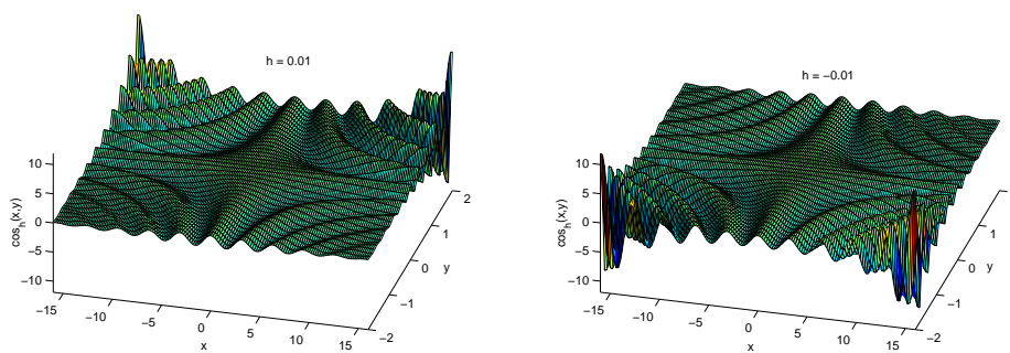
Fig. 4: Deformed trigonometric functions for h = 0.01 and h = -0.01
