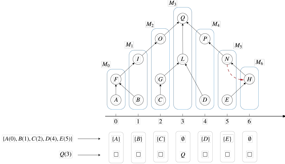
Figure 4: An execution of the automaton \mathcal{A}[\text{implies}(\Omega, \mathbf{J})] for some program \Omega and some subset \mathbf{J} of its IDB predicates. Below the timeline, we have an input word encoding an EDB stream S = \{A(0), B(1), C(2), D(4), E(5)\} and the answer fact Q(3) . Above the timeline, we have a set of facts M_0 \cup \dots \cup M_6 which encodes a derivation of Q(3) from S \cup \Omega . Each predicate X in the figure aligned with a point \tau of the timeline encodes the fact X(\tau) ; for instance, A encodes A(0) . A box labelled with M_\tau encloses the content of M_\tau ; for instance, the left-most box encodes the content \{A, F\} of M_0 . Arrows denote how IDB facts are derived from other facts, where multiple incoming arrows are to be interpreted as ‘logical and’; for instance, F(0) is derived by the rule A(0) \wedge B(1) \rightarrow F(0) . The automaton keeps track of the transitive closure of the graph induced by the derivation, and prevents cycles from appearing in the closure, so to have a well-formed derivation. For instance, when the automaton processes time 6, it may consider deriving H(6) from N(5) , but it avoids to do so because this would yield a cycle as indicated by the red dashed arrow in the figure.
