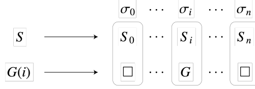
Figure 2: Encoding of fact-entailment instances as words. An instance consisting of a finite set of facts S and a fact G(i) is encoded as the word \sigma_0 \dots \sigma_n where n is the maximum between i and the largest time point occurring in S . Each symbol \sigma_j is a pair where the first component is the set of predicates S_j occurring in S \upharpoonright_j , and the second component is either the predicate G or the blank symbol \square .
