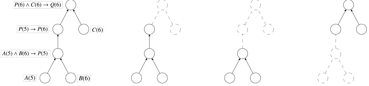
Figure 1: The first labelled tree from the left is a derivation \delta of Q(6) from \Pi \cup D with \Pi = \{A(t) \wedge B(t+1) \rightarrow P(t), P(t) \rightarrow P(t+1), P(t) \wedge C(t) \rightarrow Q(t)\} and D = \{A(5), B(6), C(6)\} . Each node has its label right next to it. Considering the same labelling for the other trees, the second tree is a P(6) -subderivation of \delta , which is also strict and immediate; the third tree is a P(5) -subderivation of \delta , which is strict but not immediate; finally, the fourth tree is a partial derivation, but not a derivation because it has no P(5) -subderivation.
