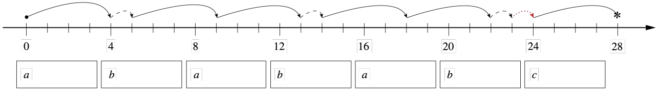
Figure 5: Pointer's moves for the expression (ab)^3c on input word abababc . Each tape cell spans 4 time points, since the exponent requires 2 bits. Solid arrows denote pointer's moves to the next cell with no change in its relative position within a cell (and hence no change in counter values). Dashed arrows denote within-cell moves, to increase the counter by one when subexpression ab has just been matched. The dotted red arrow denotes a pointer's move to the next cell with a counter reset, hence a move to the beginning of the cell. The right-most arrow, ending with an asterisk, denotes that the given SRE has been matched.
