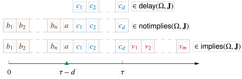
Figure 3: The delay language. A word w_1 = c_1 \dots c_d is in the language \text{delay}(\Omega, \mathbf{J}) if it can be extended to a word w_2 = b_1 \dots b_n a w_1 of \text{notimplies}(\Omega, \mathbf{J}) for a encoding an answer fact over a predicate in \mathbf{J} , and in addition w_2 can be extended to a word w_3 = w_2 v_1 \dots v_m of \text{implies}(\Omega, \mathbf{J}) . This means that w_3 encodes a stream S and a fact \alpha holding at \tau - d such that \Omega \cup S \models \alpha , and w_2 encodes that \Omega \cup S \upharpoonright_{[0, \tau]} \not\models \alpha . Thus, the length d of w_1 is not a valid delay for \Omega , and hence words in \text{delay}(\Omega, \mathbf{J}) witness the non-validity of delays via their length.
