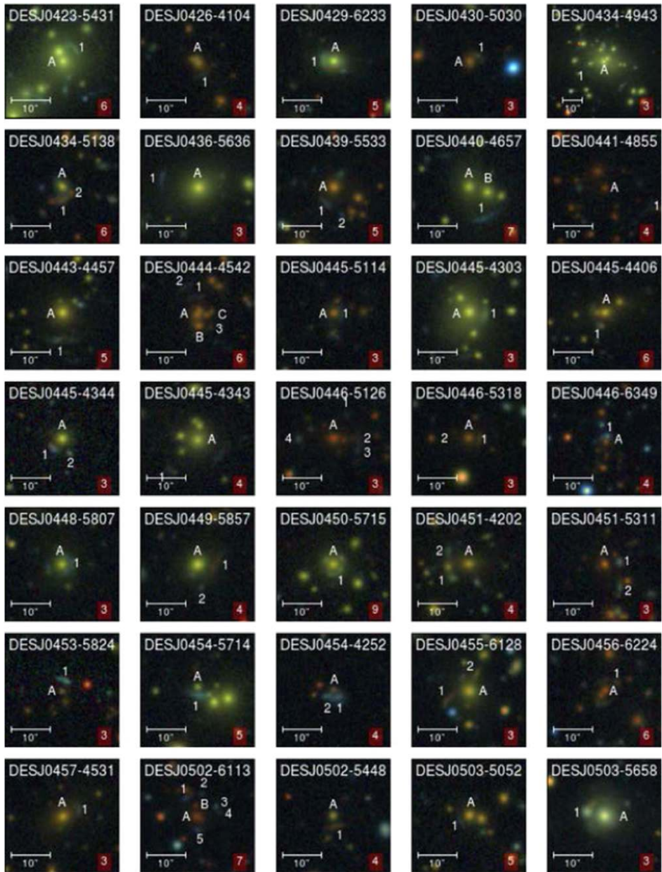
Figure 11. Sixth page of SL systems with ranks of 3 or more. Each cutout image has the visual inspection ranking displayed in a red box in the lower right hand corner. All images are oriented with north up and east left. Most of the cutouts are 30'' \times 30'' in size. Some of the largest systems are displayed with 60'' \times 60'' images, so that they fit well within the cutout. A scale bar 10'' long is displayed in the lower left hand corner.
