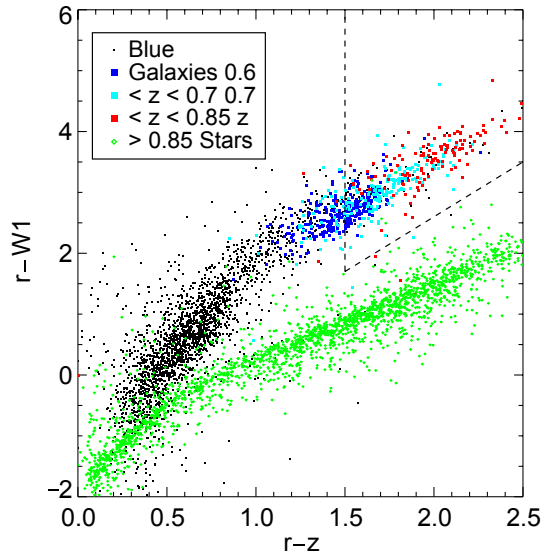
Figure 3.6: An optical/near-infrared color-color diagram for galaxies observed by both DECAM and WISE in the COSMOS field, where highly accurate 30-band photometric redshifts are available and used to label the points shown. In this and subsequent figures, r indicates DECAM r -band AB magnitude, z indicates DECAM z_{AB} , and W1 indicates WISE 3.4 \mu\text{m} AB magnitude. Galaxies with LRG-like spectral energy distributions also having z > 0.6 are indicated by points color-coded according to their redshift, whereas small black points indicate blue galaxies at all redshifts. The dashed lines indicate the borders of our LRG selection box; our baseline sample assumes that objects above and to the right of these lines that also have magnitude z_{AB} < 20.46 will be targeted by DESI as high-redshift LRGs.
