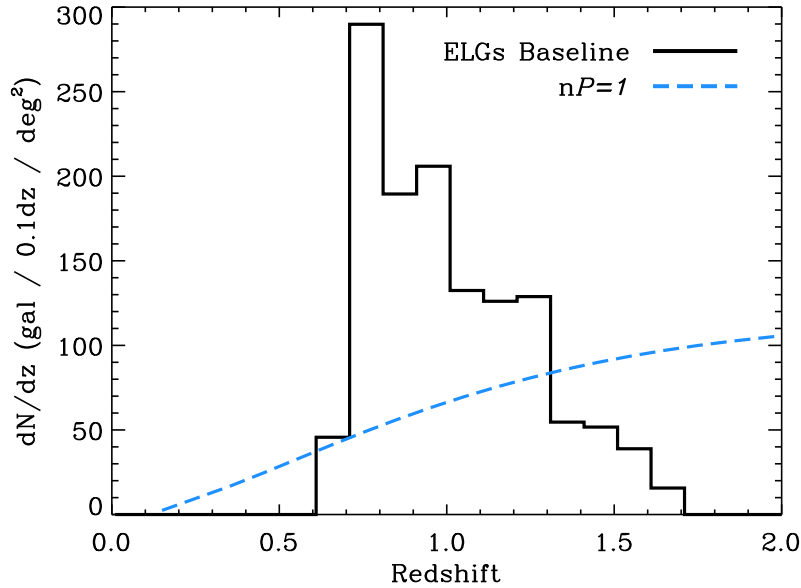
Figure 3.12: Expected redshift distribution of ELG targets based on our analysis of the DEEP2/EGS survey data (see Figure 3.10). The overall normalization of the distribution has been fixed to 1280 ELGs \text{deg}^{-2} (from a targeted sample of 2400 targets \text{deg}^{-2} ) to reflect conservative estimates of the overall efficiencies of fiber assignment, target selection, and redshift measurement. The ELG redshift distribution drops to a level where shot noise dominates errors in BAO measurements (i.e., \bar{n}P < 1 ) only at z \gtrsim 1.3 (dashed blue line).
