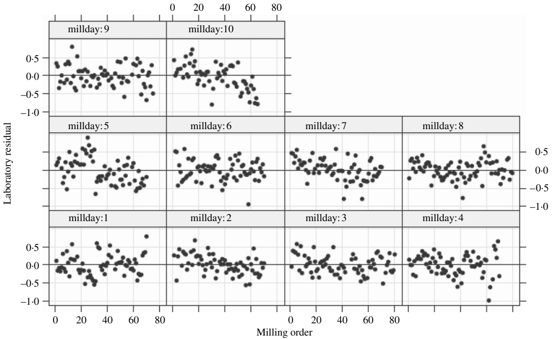
Fig. 2. Analysis of DH-5 trial: estimated laboratory residuals from model M1 graphed against milling order for each milling day.
