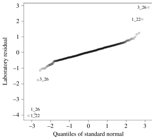
Fig. 1. Analysis of DH-5 trial: QQ-plot for estimated laboratory residuals from model M0. Potential outliers are labelled with their field column and row numbers.
