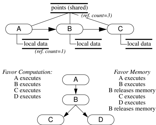
Figure 6 Memory management. (top) reference counting, (bottom) memory/computation trade-off
