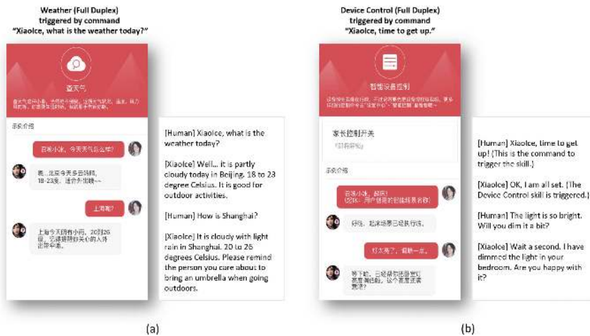
Figure 19 Examples of Task Completion skills, their triggers with users in Chinese (left) and English translation (right). (a) The Weather skill, triggered by the command “XiaoIce, what is the weather today.” (b) The Device Control (Full Duplex) skill, triggered by the command “XiaoIce, time to get up.”
